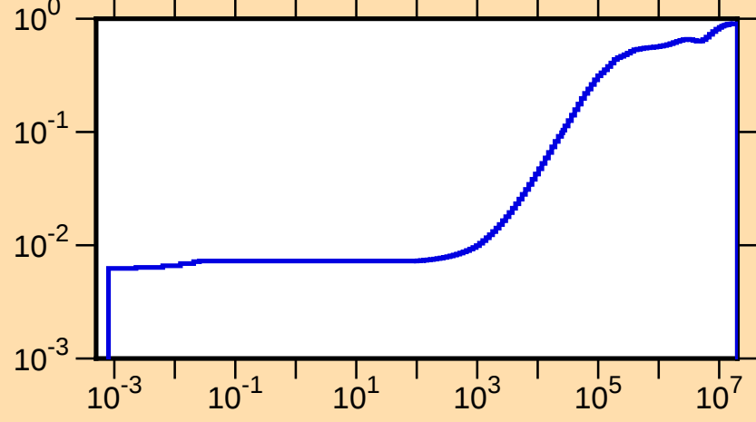
\mu vs. E for ^{109}\text{Sb}(\text{mt251})
