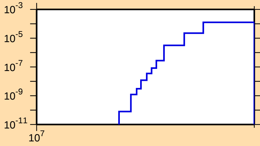
\sigma vs. E for ^{109}\text{Sb}(n,\text{nd})
