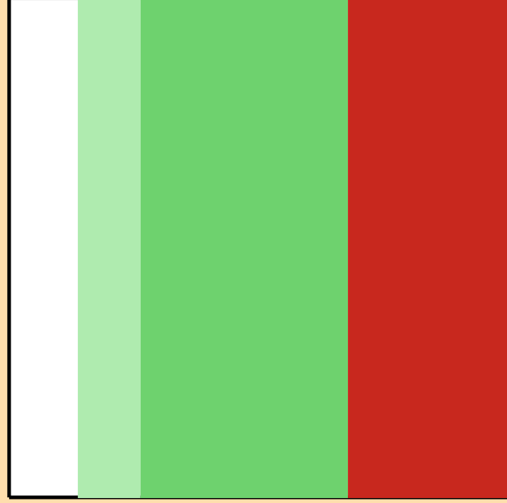
\Delta\sigma/\sigma vs. E for ^{109}\text{Sb}(n,2n)
