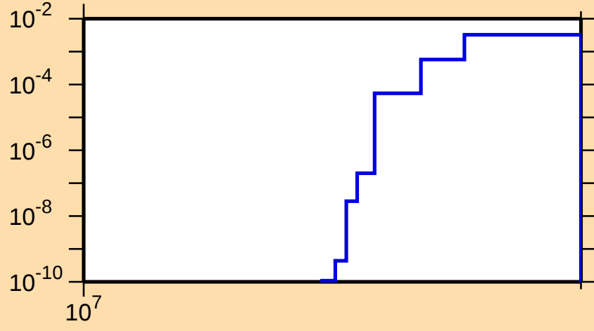
\sigma vs. E for ^{109}\text{Sb}(n,2np)
