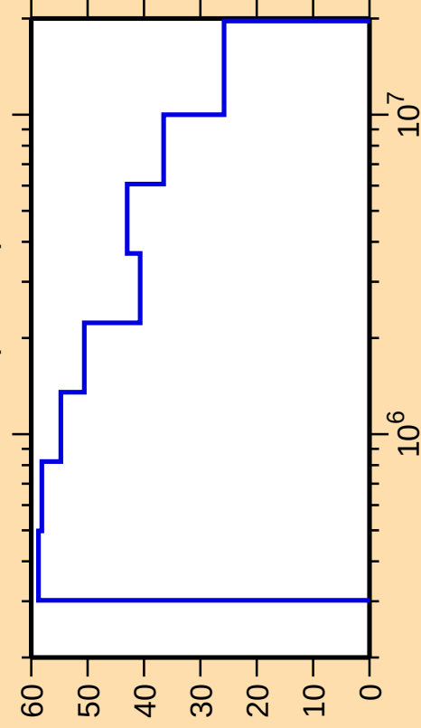
\Delta\sigma/\sigma vs. E for ^{109}\text{Sb}(n,\text{inel.})
