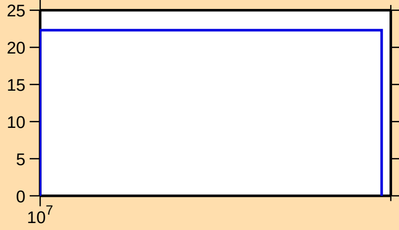
\Delta\sigma/\sigma vs. E for ^{109}\text{Sb}(n,\text{el.})
