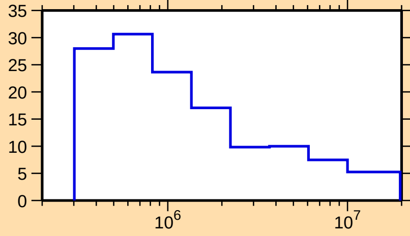
\Delta\sigma/\sigma vs. E for ^{109}\text{Sb}(n,\text{nonel.})
