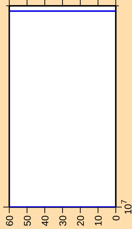
\Delta\sigma/\sigma vs. E for ^{109}\text{Sb}(n,p)
