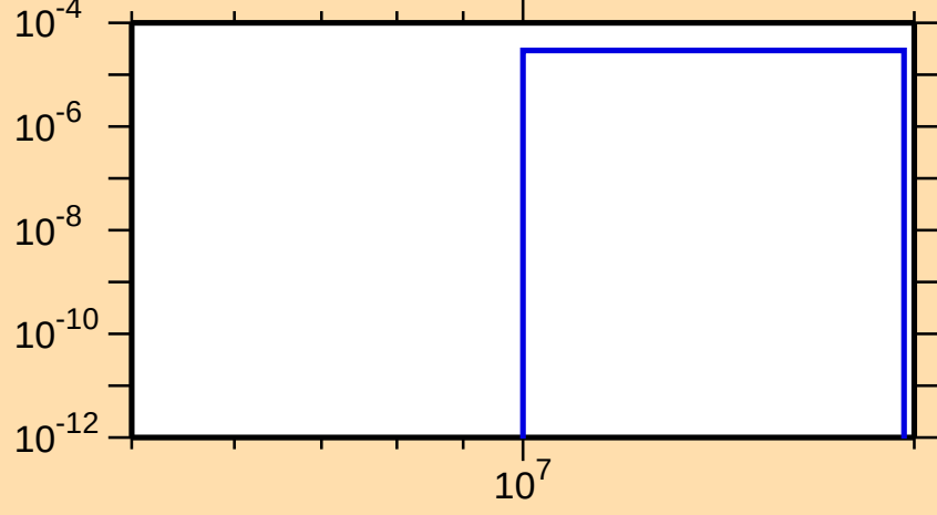
\sigma vs. E for ^{109}\text{Sb}(\text{mt } 45)
