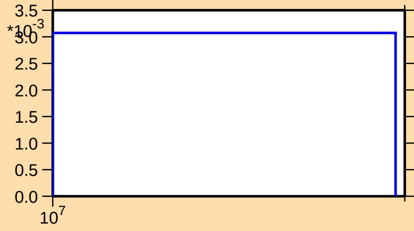
\sigma vs. E for ^{109}\text{Sb}(n,2n)
