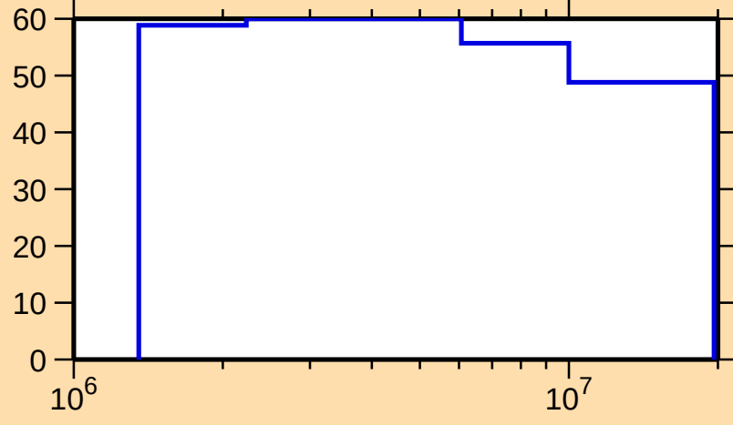
\Delta\sigma/\sigma vs. E for ^{109}\text{Sb}(n,n_1)
