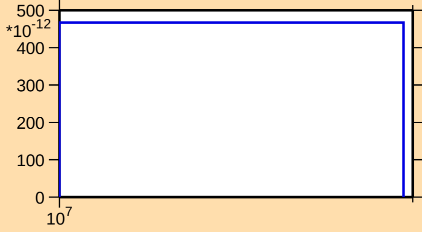
\sigma vs. E for ^{109}\text{Sb}(n,2n\alpha)
