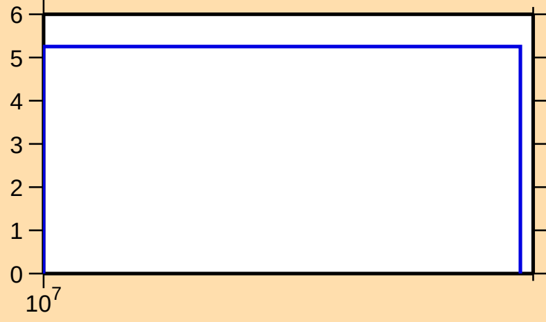
\Delta\sigma/\sigma vs. E for ^{109}\text{Sb}(n,\text{nonel.})
