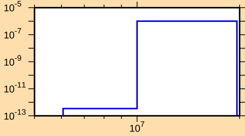
\sigma vs. E for ^{109}\text{Sb}(\text{mt117})
