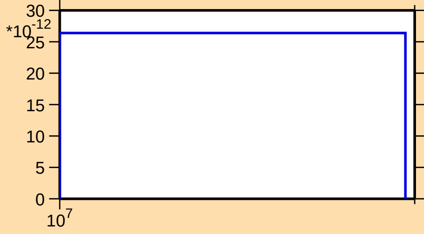
\sigma vs. E for ^{109}\text{Sb}(\text{mt } 34)
