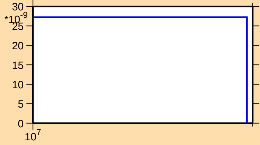
\sigma vs. E for ^{109}\text{Sb}(n,\text{pt})
