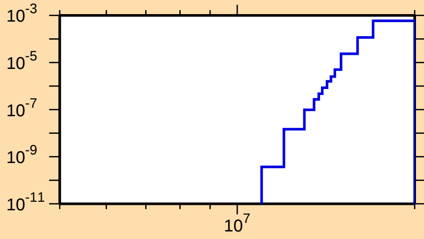
\sigma vs. E for ^{110}\text{Sb}(\text{mt } 45)
