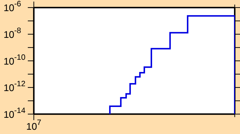
\sigma vs. E for ^{110}\text{Sb}(\text{mt } 34)
