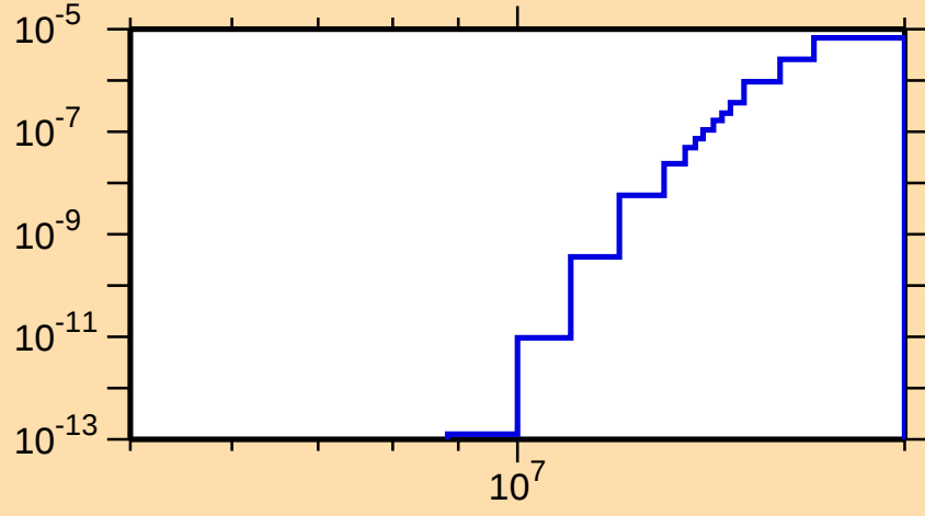
\sigma vs. E for ^{110}\text{Sb}(\text{mt117})
