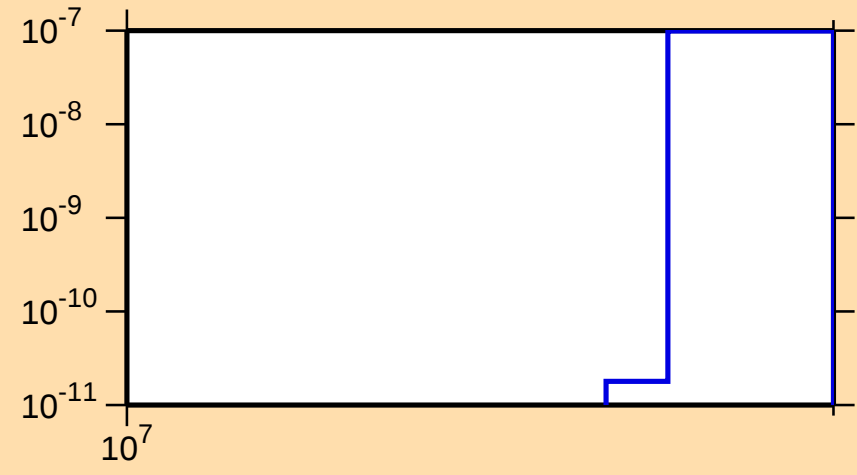
\sigma vs. E for ^{110}\text{Sb}(n,nt)
