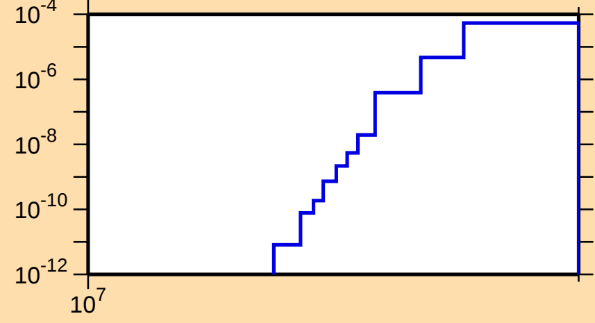
\sigma vs. E for ^{110}\text{Sb}(n,\text{pt})
