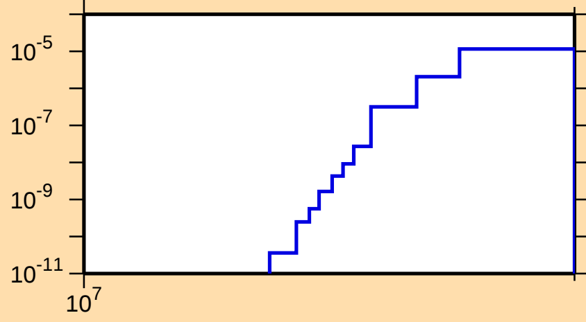
\sigma vs. E for ^{110}\text{Sb}(n,2n\alpha)
