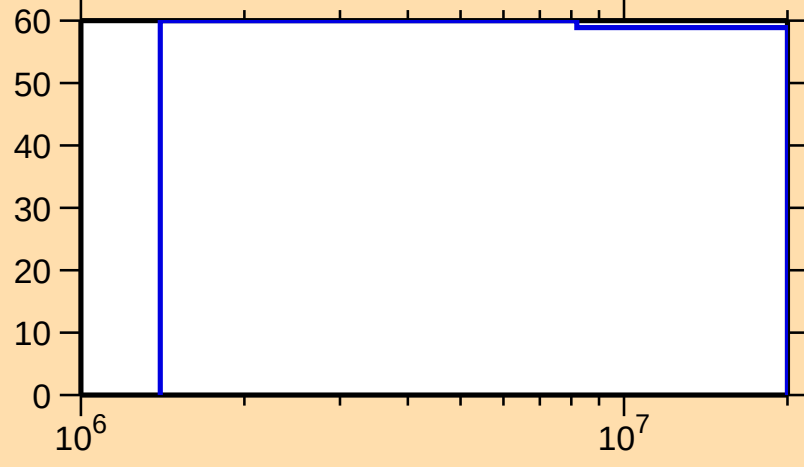
\Delta\sigma/\sigma vs. E for ^{110}\text{Sb}(n,n_1)
