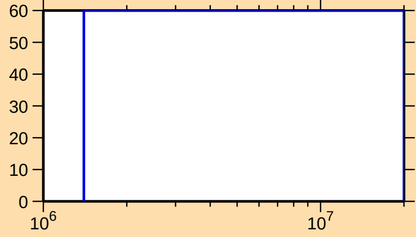
\Delta\sigma/\sigma vs. E for ^{110}\text{Sb}(n,n\text{cont.})
