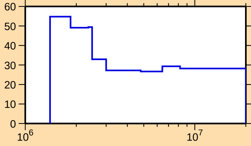
\Delta\sigma/\sigma vs. E for ^{110}\text{Sb}(n,n\text{nonel.})
