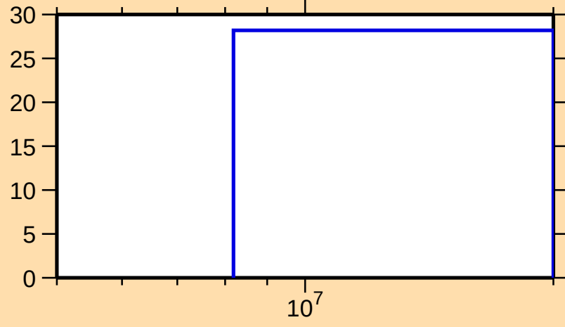
\Delta\sigma/\sigma vs. E for ^{110}\text{Sb}(n,\text{nonel.})
