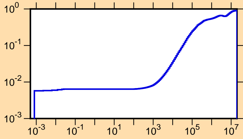
\mu vs. E for ^{118}\text{Sb}(\text{mt251})
