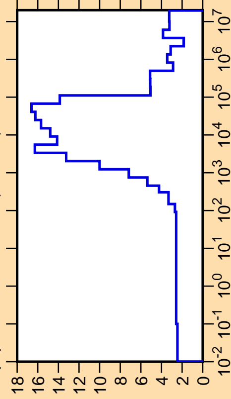
\Delta\mu/\mu vs. E for ^{118}\text{Sb}(\text{mt251})
