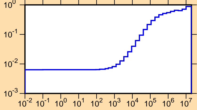
\mu vs. E for ^{118}\text{Sb}(\text{mt251})
