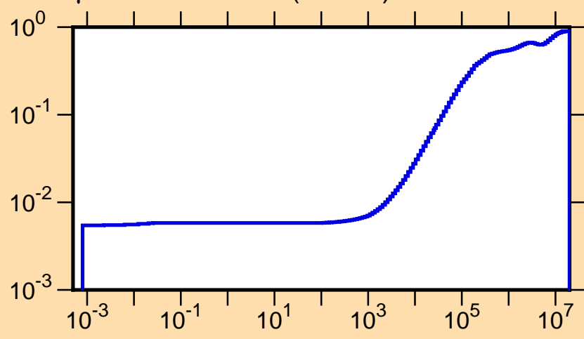
\mu vs. E for ^{124}\text{Sb}(\text{mt251})
