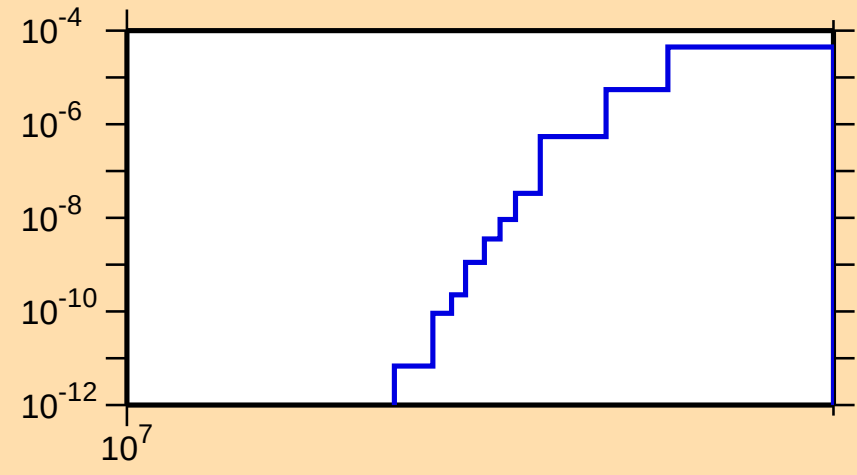
\sigma vs. E for ^{124}\text{Sb}(n,nd)
