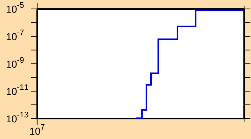
\sigma vs. E for ^{124}\text{Sb}(n,2np)
