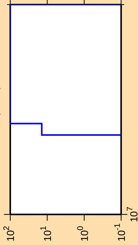
\Delta\sigma/\sigma vs. E for ^{124}\text{Sb}(n,nd)
