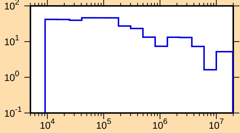
\Delta\sigma/\sigma vs. E for ^{124}\text{Sb}(n,\text{tot.})
