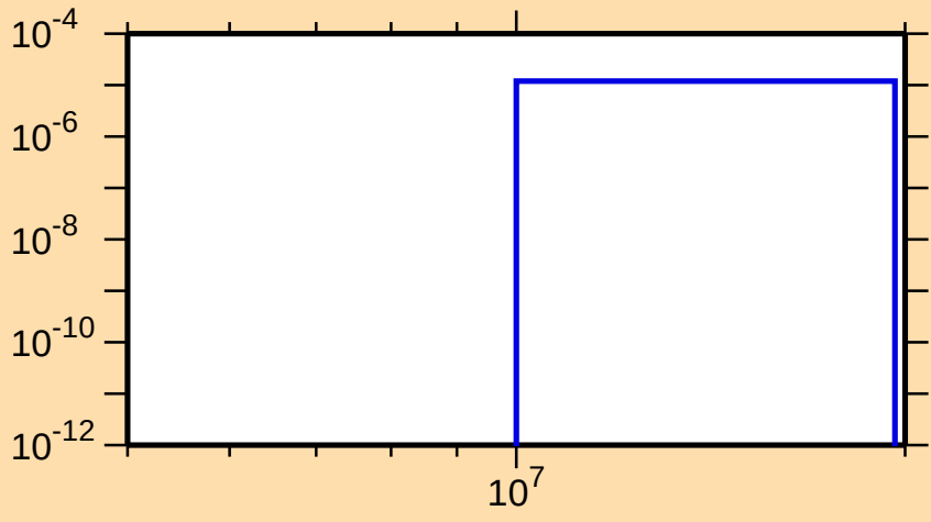
\sigma vs. E for ^{124}\text{Sb}(n,n\alpha)
