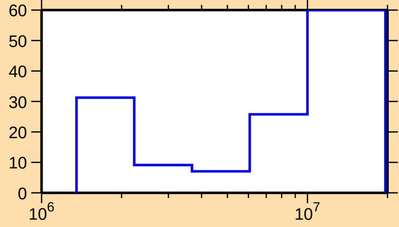
\Delta\sigma/\sigma vs. E for ^{124}\text{Sb}(n,n\text{cont.})
