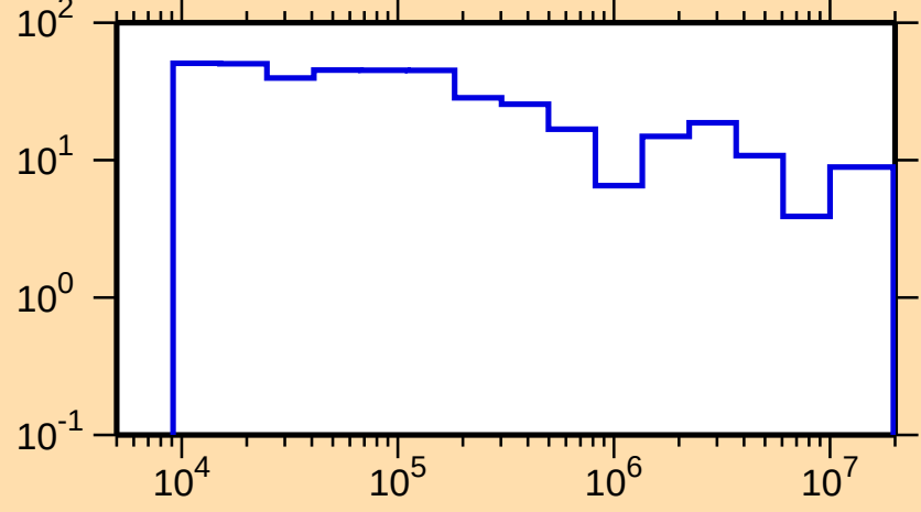
\Delta\sigma/\sigma vs. E for ^{124}\text{Sb}(n,\text{el.})
