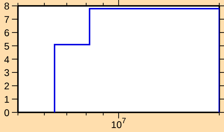
\Delta\sigma/\sigma vs. E for ^{124}\text{Sb}(n,\text{el.})
