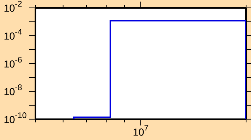
\sigma vs. E for ^{124}\text{Sb}(n,d)
