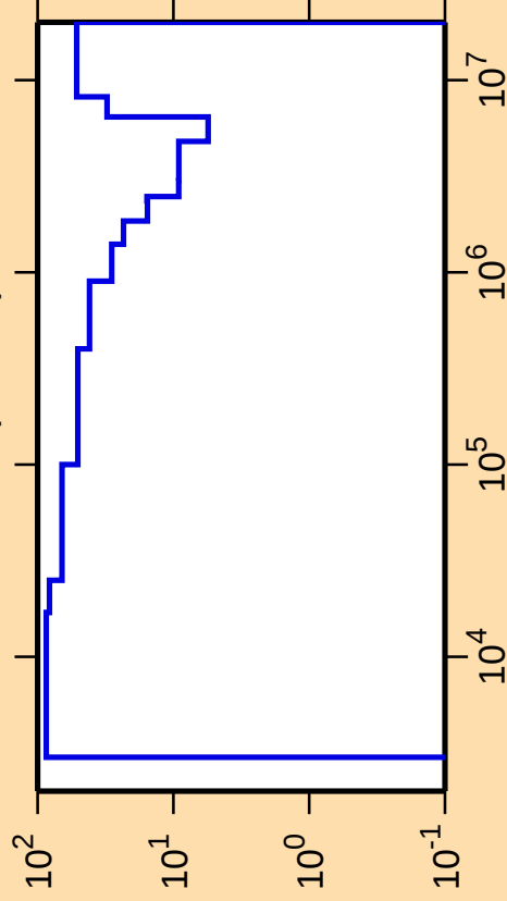
\Delta\sigma/\sigma vs. E for ^{124}\text{Sb}(n,\text{inel.})
