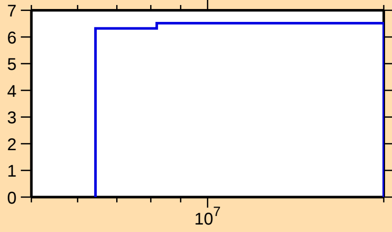
\Delta\sigma/\sigma vs. E for ^{124}\text{Sb}(n,\text{nonel.})
