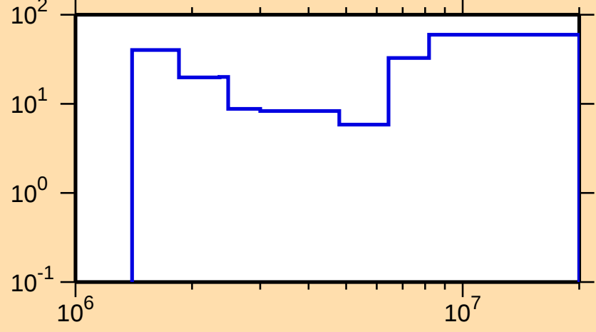
\Delta\sigma/\sigma vs. E for ^{124}\text{Sb}(n,n\text{cont.})
