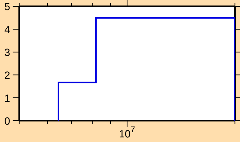
\Delta\sigma/\sigma vs. E for ^{124}\text{Sb}(n,\text{tot.})
