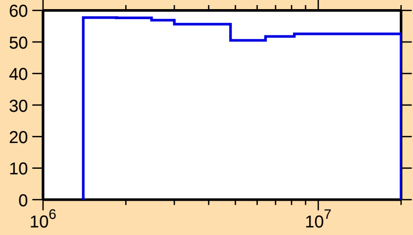
\Delta\sigma/\sigma vs. E for ^{124}\text{Sb}(n,p)
