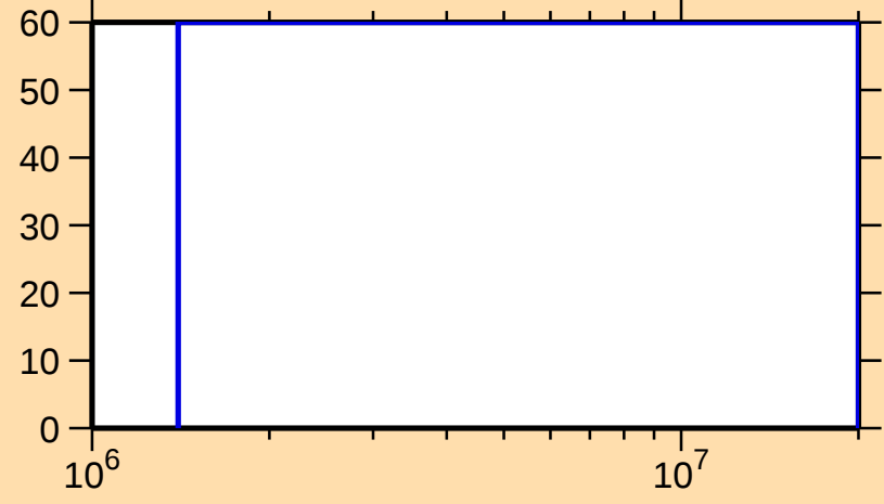
\Delta\sigma/\sigma vs. E for ^{124}\text{Sb}(n,n_1)
