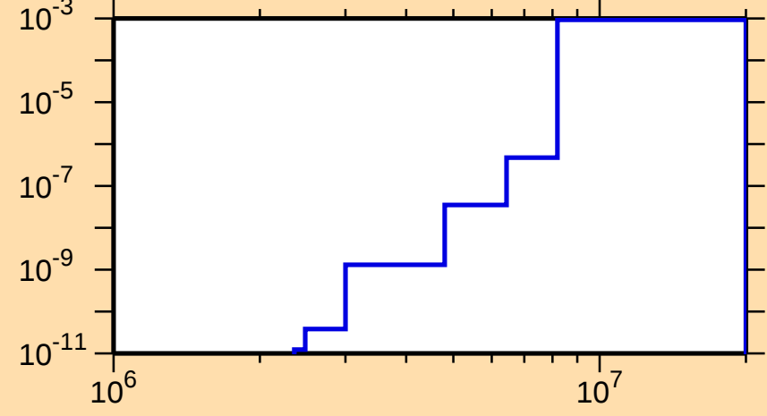
\sigma vs. E for ^{124}\text{Sb}(n,\alpha)
