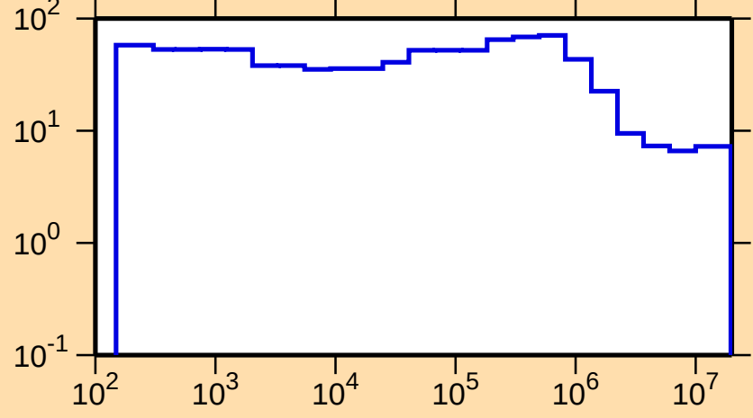
\Delta\sigma/\sigma vs. E for ^{124}\text{Sb}(n,\text{nonel.})
