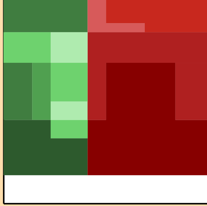
\Delta\sigma/\sigma vs. E for ^{129}\text{Sb}(n,\text{tot.})
