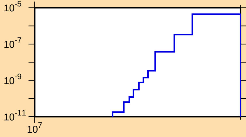
\sigma vs. E for ^{129}\text{Sb}(n,n\alpha)
