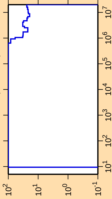
\Delta\sigma/\sigma vs. E for ^{129}\text{Sb}(n,\text{nonel.})
