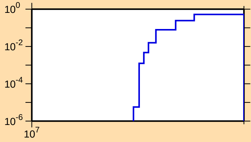
\sigma vs. E for ^{129}\text{Sb}(n,3n)
