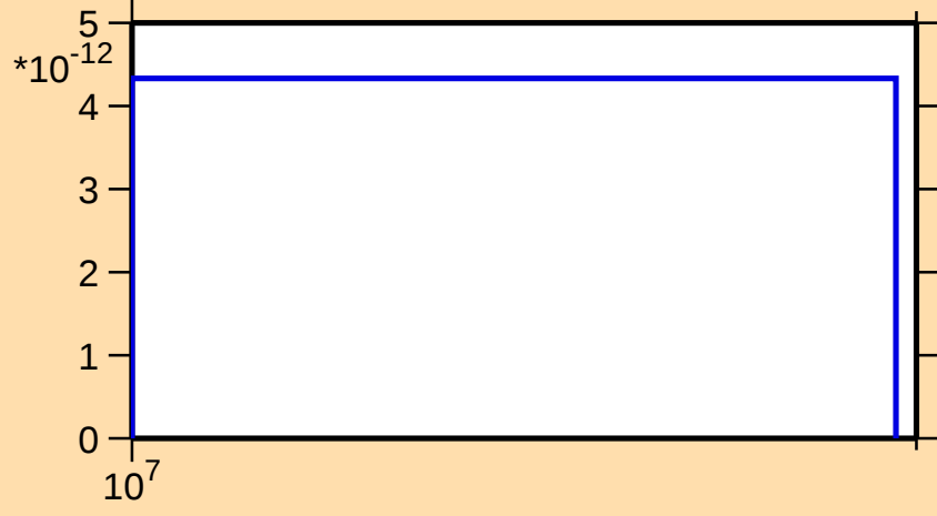
\sigma vs. E for ^{129}\text{Sb}(n,2np)
