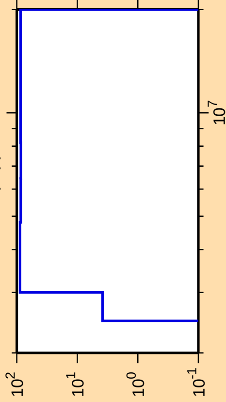
\Delta\sigma/\sigma vs. E for ^{130}\text{Sb}(n,p)
