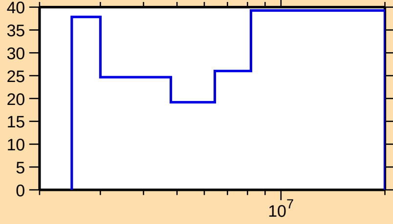
\Delta\sigma/\sigma vs. E for ^{130}\text{Sb}(n,n\text{cont.})
