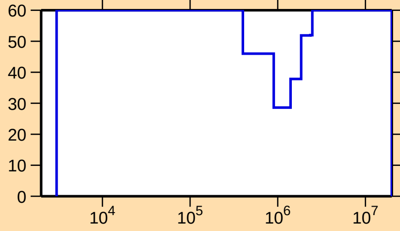
\Delta\sigma/\sigma vs. E for ^{130}\text{Sb}(n,n_1)
