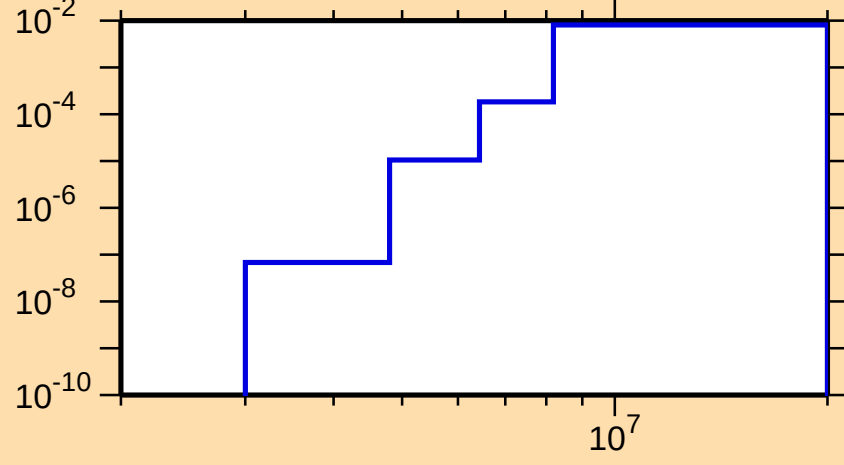
\sigma vs. E for ^{130}\text{Sb}(n,p)
