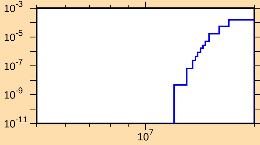
\sigma vs. E for ^{42}\text{Sc}(\text{mt117})
