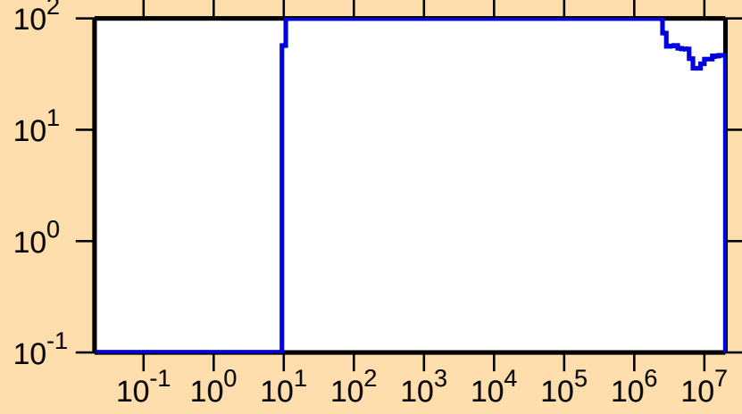
\Delta\sigma/\sigma vs. E for ^{42}\text{Sc}(n,\gamma)
