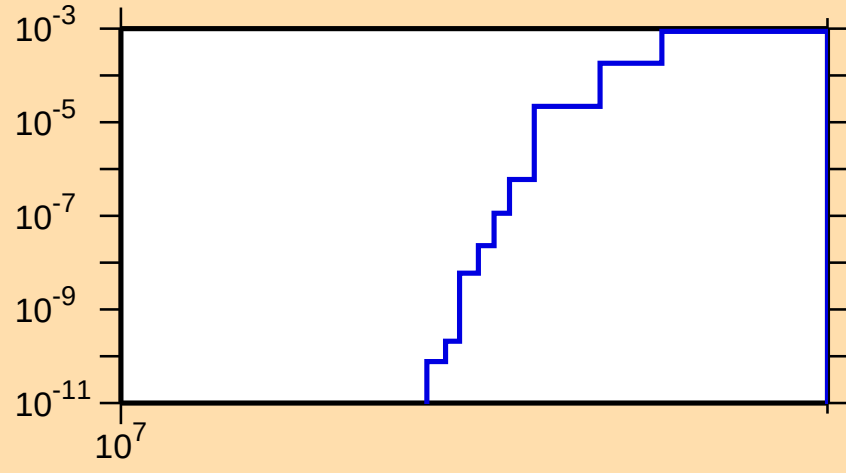
\sigma vs. E for ^{42}\text{Sc}(n,\text{pt})
