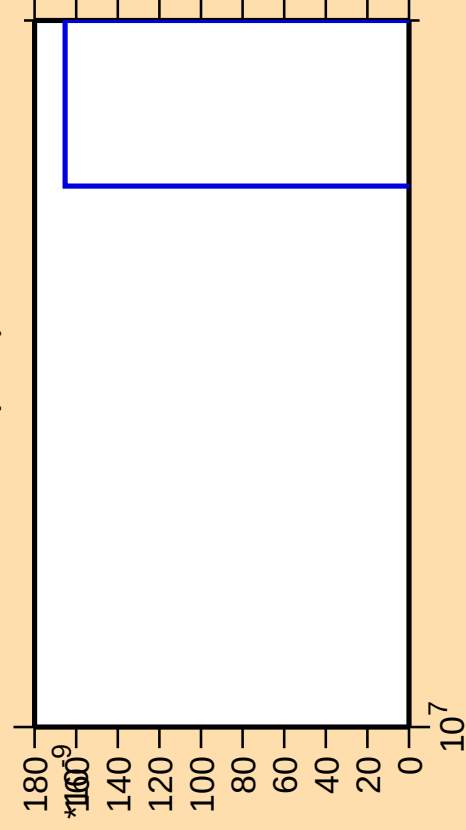
\Delta\sigma/\sigma vs. E for ^{42}\text{Sc}(n,nt)
