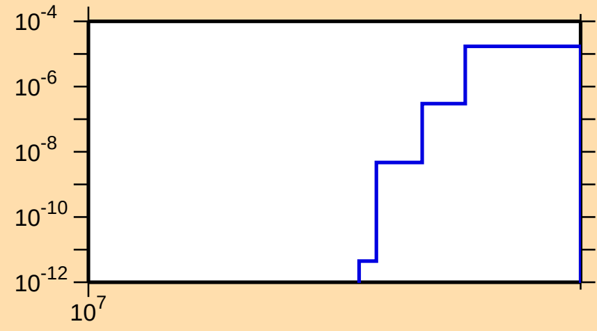
\sigma vs. E for ^{42}\text{Sc}(\text{mt } 34)
