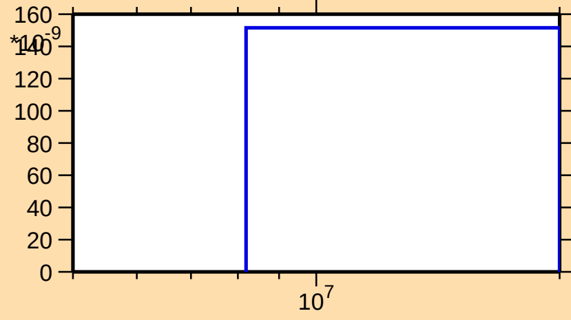
\sigma vs. E for ^{42}\text{Sc}(\text{mt } 34)
