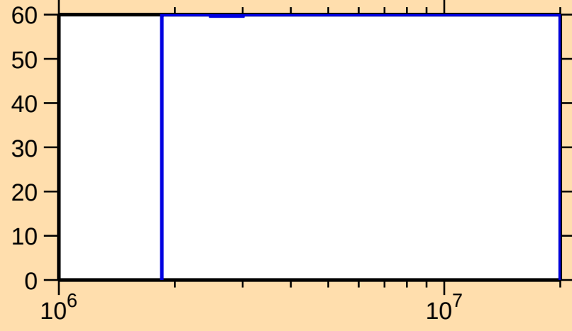
\Delta\sigma/\sigma vs. E for ^{42}\text{Sc}(n,n_1)
