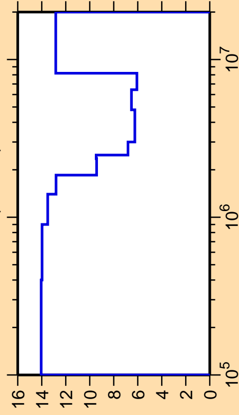
\sigma vs. E for ^{45}\text{Sc}(n,\text{inel.})
