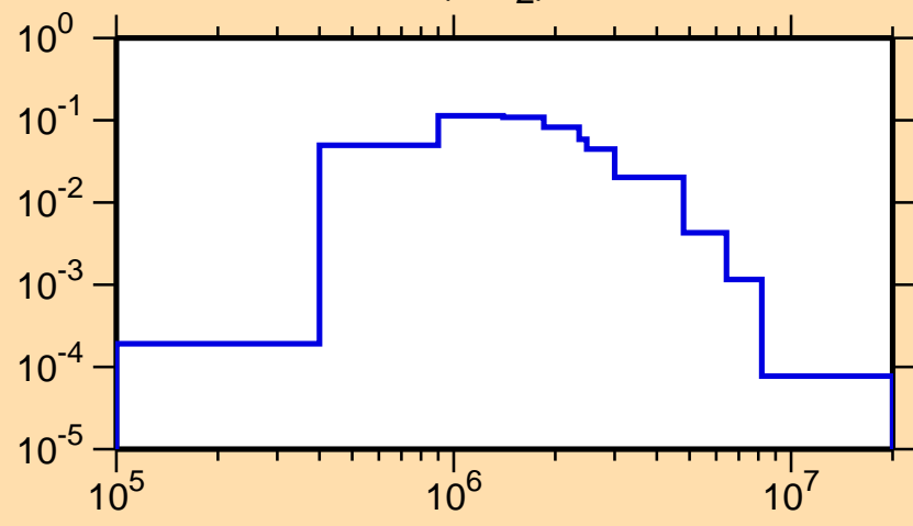
\sigma vs. E for ^{45}\text{Sc}(n,n_2)
