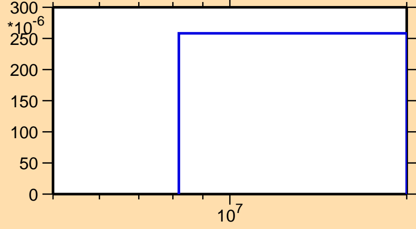
\sigma vs. E for ^{45}\text{Sc}(n,t)
