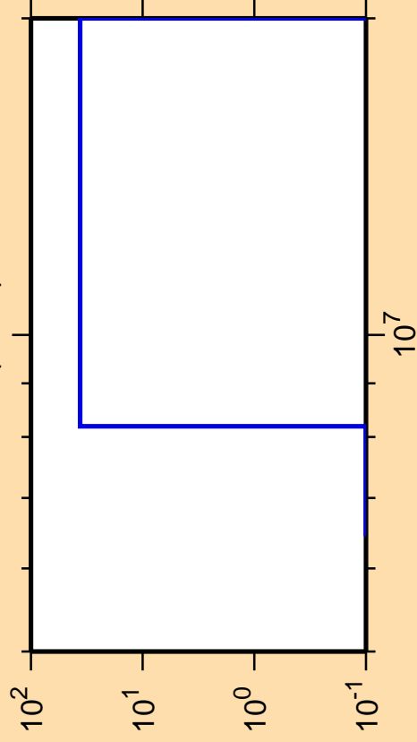
\Delta\sigma/\sigma vs. E for ^{45}\text{Sc}(n,\alpha)
