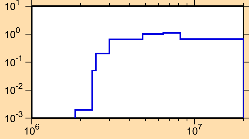
\sigma vs. E for ^{45}\text{Sc}(n,n\text{cont.})
