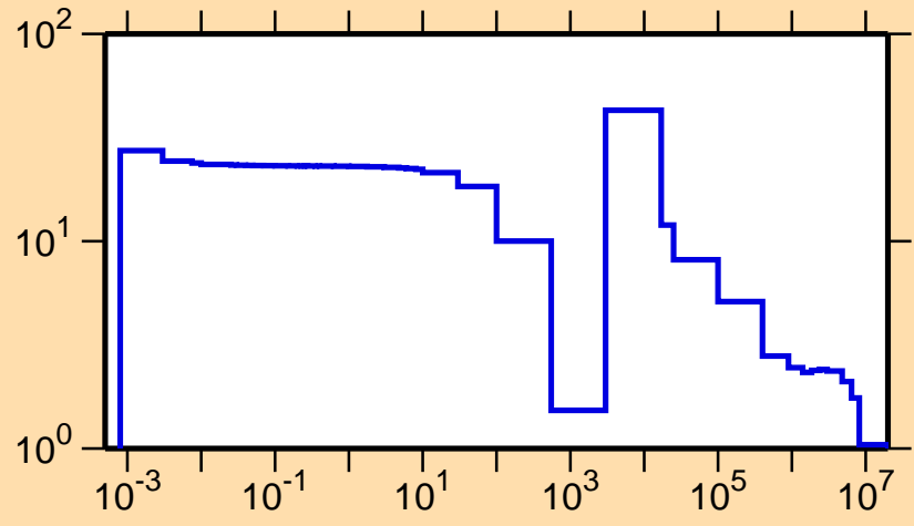
\sigma vs. E for ^{45}\text{Sc}(n,\text{el.})
