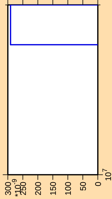
\Delta\sigma/\sigma vs. E for ^{49}\text{Sc}(n,p\alpha)
