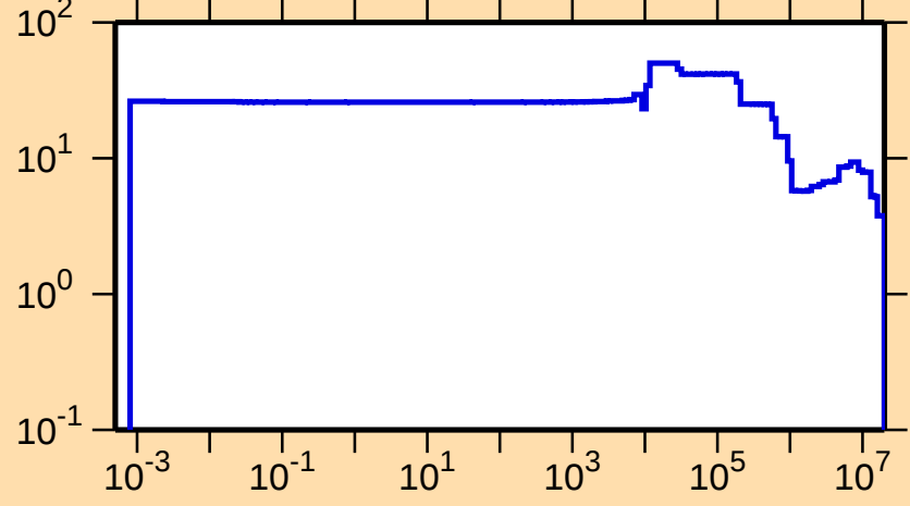
\Delta\sigma/\sigma vs. E for ^{49}\text{Sc}(n,\text{tot.})
