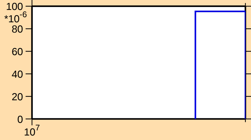
\sigma vs. E for ^{49}\text{Sc}(n,3n)
