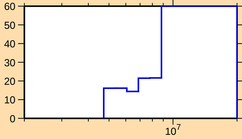
\Delta\sigma/\sigma vs. E for ^{49}\text{Sc}(n,n_1)
