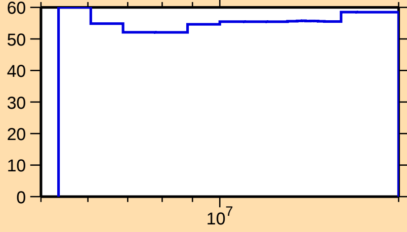
\Delta\sigma/\sigma vs. E for ^{49}\text{Sc}(n,p)
