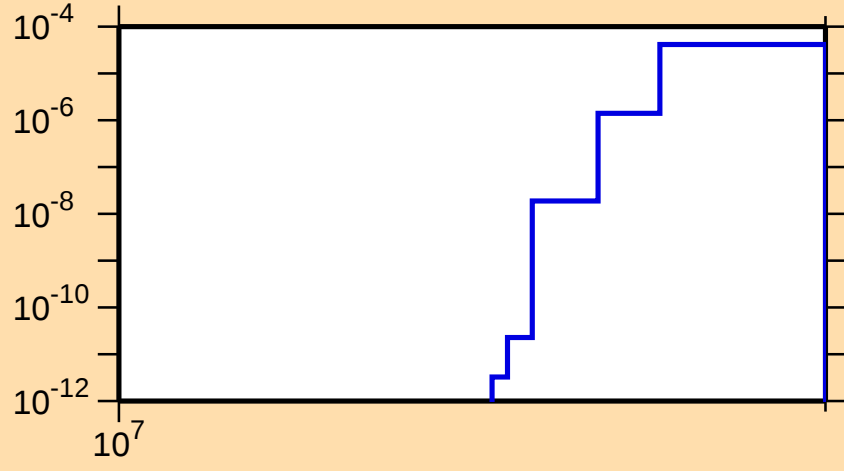
\sigma vs. E for ^{49}\text{Sc}(n,n\alpha)
