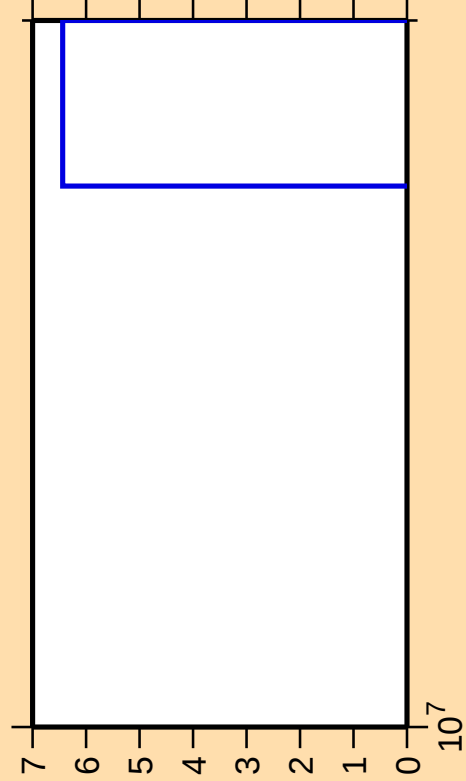
\Delta\sigma/\sigma vs. E for ^{49}\text{Sc}(n,nt)
