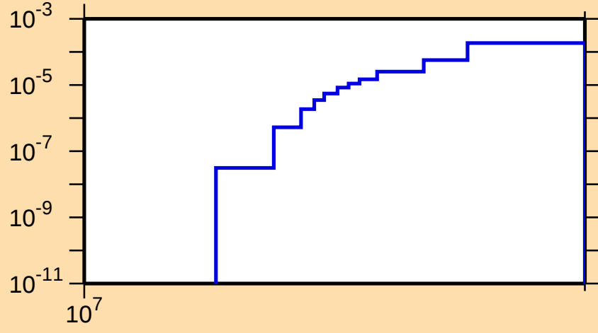
\sigma vs. E for ^{49}\text{Sc}(n,t)
