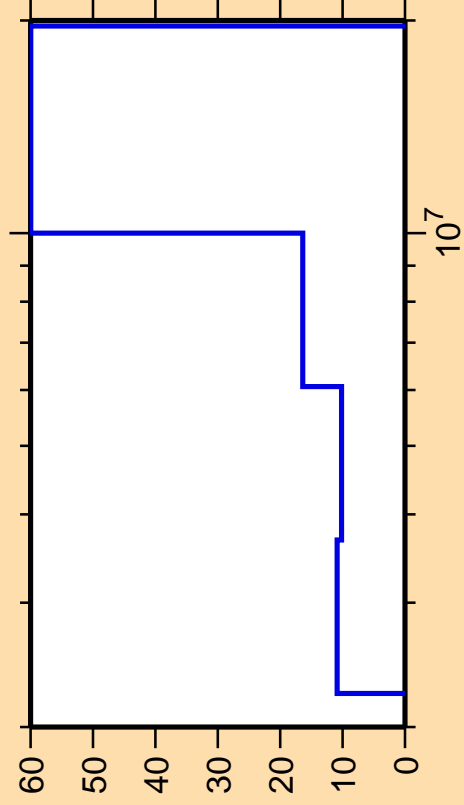
\Delta\sigma/\sigma vs. E for ^{49}\text{Sc}(n,n_4)
