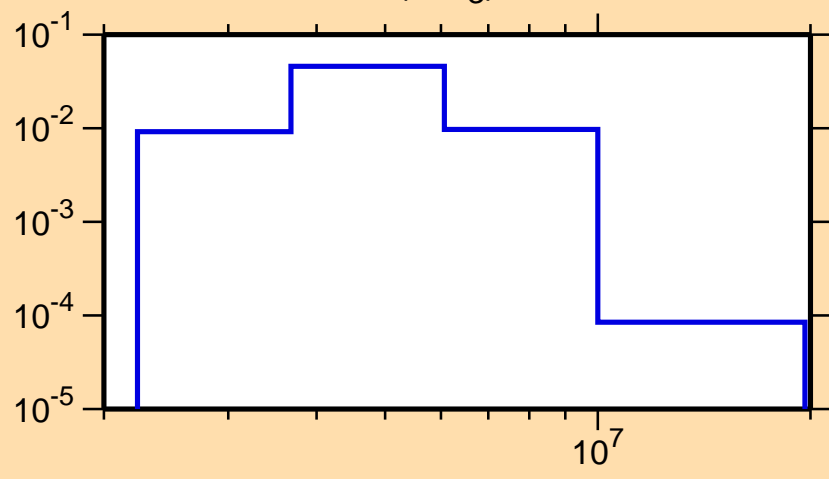
\sigma vs. E for ^{49}\text{Sc}(n,n_3)
