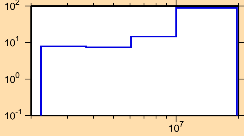
\Delta\sigma/\sigma vs. E for ^{49}\text{Sc}(n,n_1)
