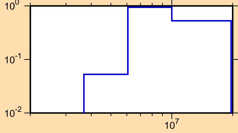
\sigma vs. E for ^{49}\text{Sc}(n,n\text{cont.})
