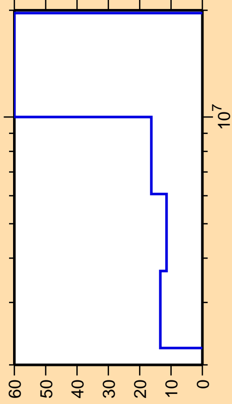
\Delta\sigma/\sigma vs. E for ^{49}\text{Sc}(n,n_3)
