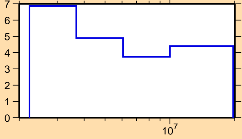
\Delta\sigma/\sigma vs. E for ^{49}\text{Sc}(n,\text{nonel.})
