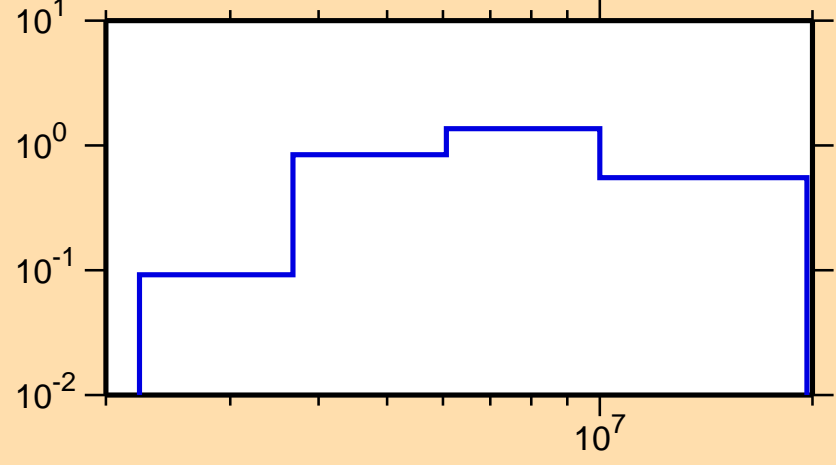
\sigma vs. E for ^{49}\text{Sc}(n,\text{inel.})
