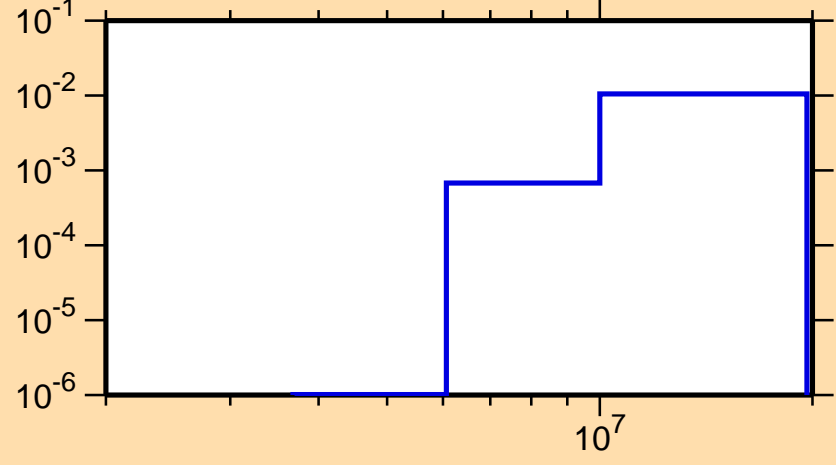
\sigma vs. E for ^{49}\text{Sc}(n,p)
