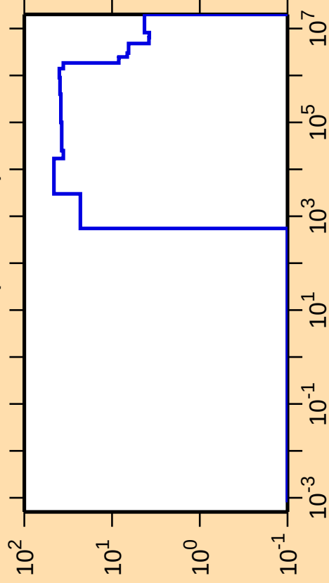
\Delta\sigma/\sigma vs. E for ^{49}\text{Sc}(n,\text{nonel.})
