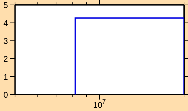
\Delta\sigma/\sigma vs. E for ^{49}\text{Sc}(n,\text{nonel.})
