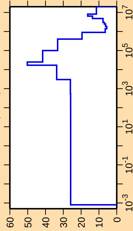
\Delta\sigma/\sigma vs. E for ^{49}\text{Sc}(n,\text{el.})
