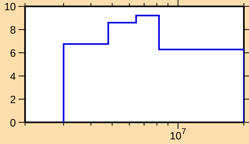
\Delta\sigma/\sigma vs. E for ^{49}\text{Sc}(n,\text{tot.})
