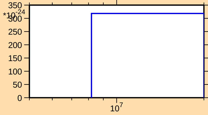
\sigma vs. E for ^{49}\text{Sc}(n,p\alpha)
