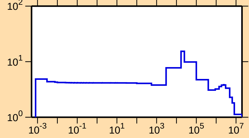
\sigma vs. E for ^{49}\text{Sc}(n,\text{el.})
