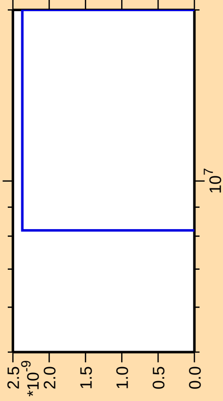
\Delta\sigma/\sigma vs. E for ^{49}\text{Sc}(n,p\alpha)
