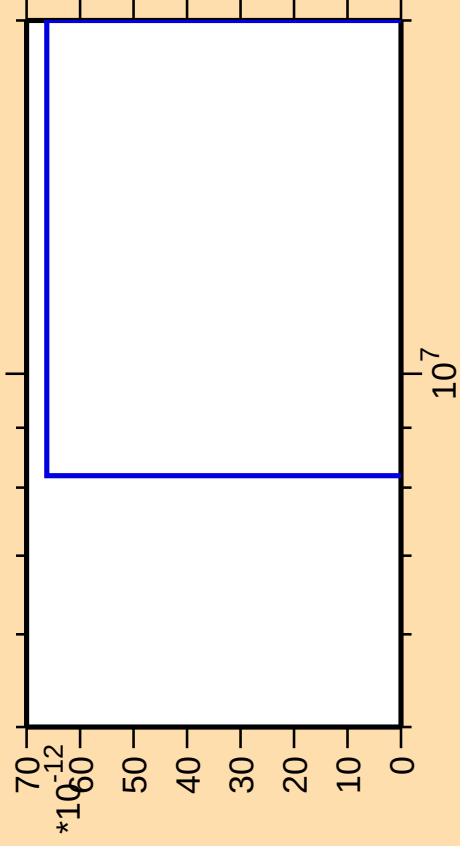
\Delta\sigma/\sigma vs. E for ^{49}\text{Sc}(n,2np)
