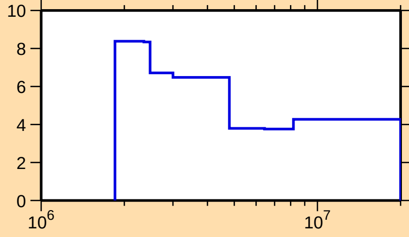
\Delta\sigma/\sigma vs. E for ^{49}\text{Sc}(n,\text{nonel.})
