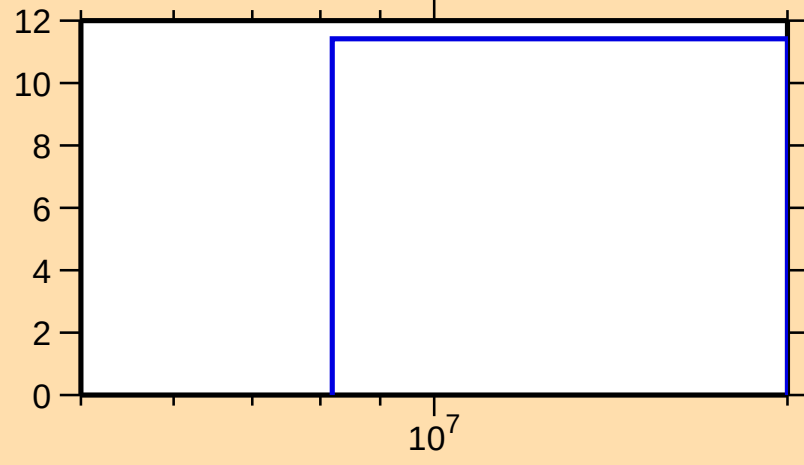
\Delta\sigma/\sigma vs. E for ^{49}\text{Sc}(n,\text{el.})
