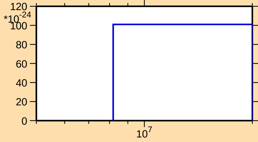
\sigma vs. E for ^{49}\text{Sc}(n,2np)
