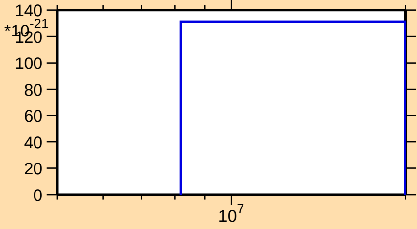
\sigma vs. E for ^{49}\text{Sc}(n,\text{He}3)
