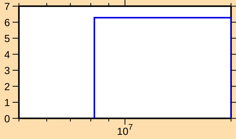
\Delta\sigma/\sigma vs. E for ^{49}\text{Sc}(n,\text{tot.})
