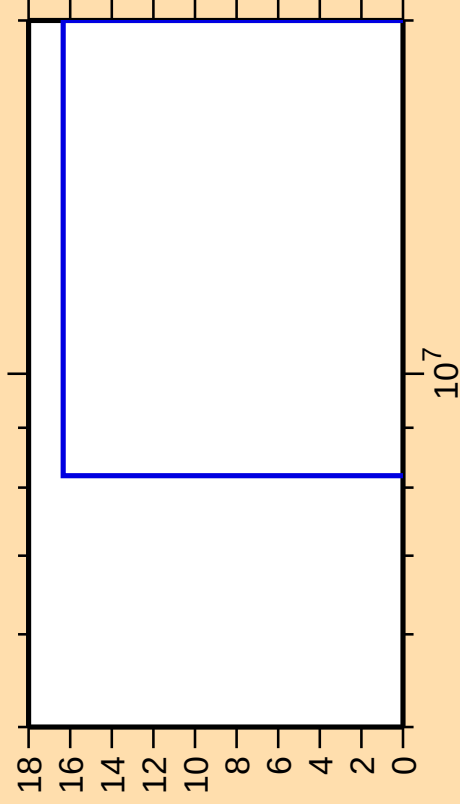
\Delta\sigma/\sigma vs. E for ^{49}\text{Sc}(n,2n)
