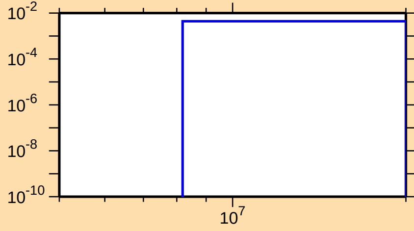
\sigma vs. E for ^{49}\text{Sc}(n,d)
