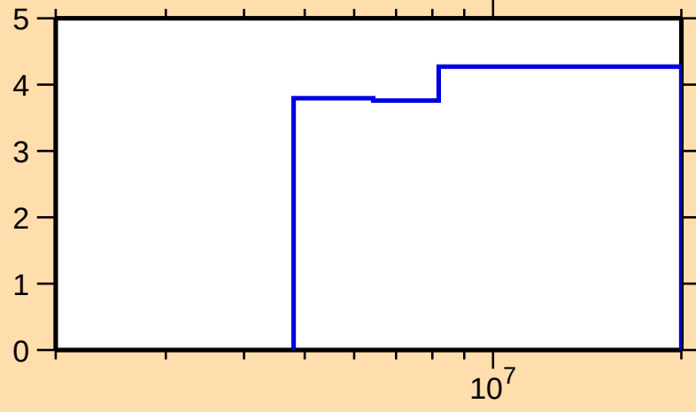
\Delta\sigma/\sigma vs. E for ^{49}\text{Sc}(n,n\text{onrel.})
