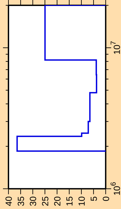
\Delta\sigma/\sigma vs. E for ^{49}\text{Sc}(n,\text{inel.})
