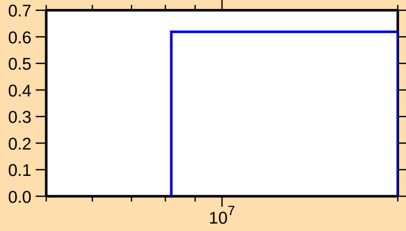
\sigma vs. E for ^{49}\text{Sc}(n,2n)
