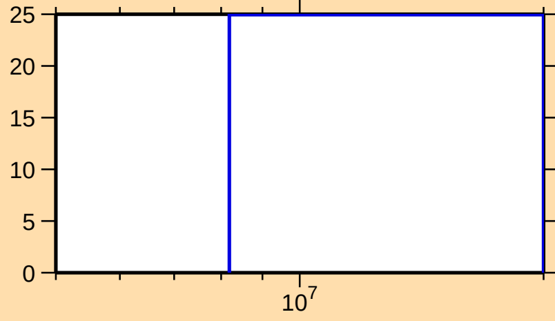
\Delta\sigma/\sigma vs. E for ^{49}\text{Sc}(n,\text{inel.})
