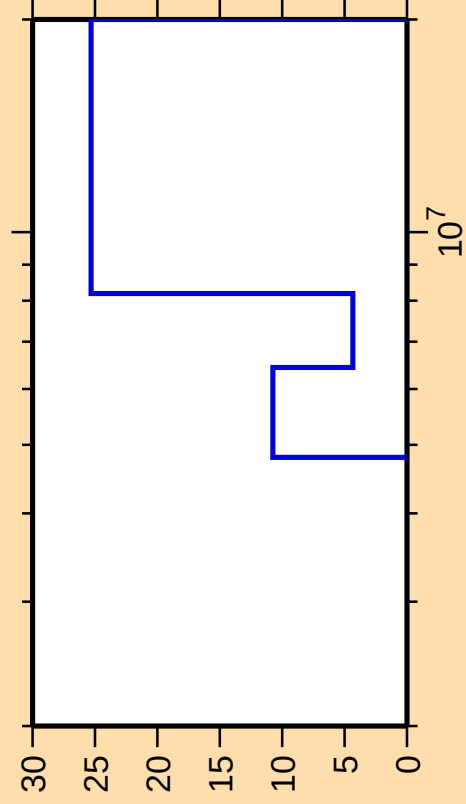
\Delta\sigma/\sigma vs. E for ^{49}\text{Sc}(n,n\text{cont.})
