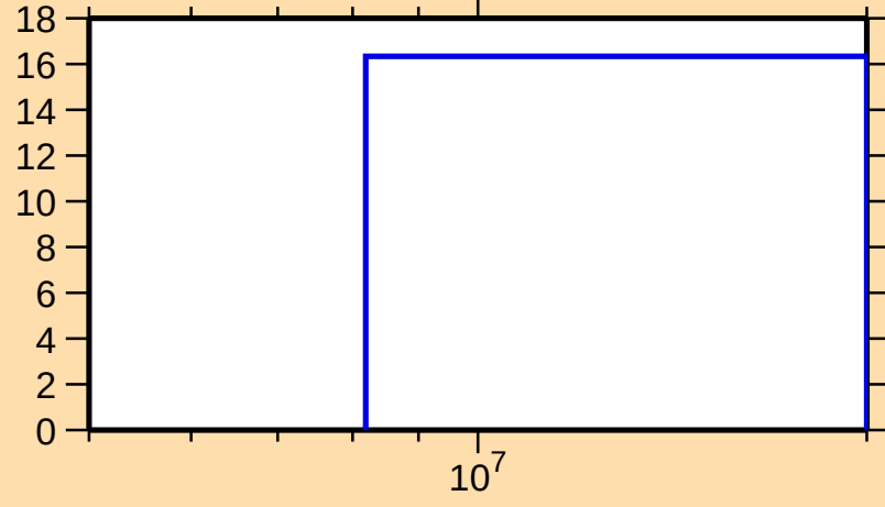
\Delta\sigma/\sigma vs. E for ^{49}\text{Sc}(n,2n)
