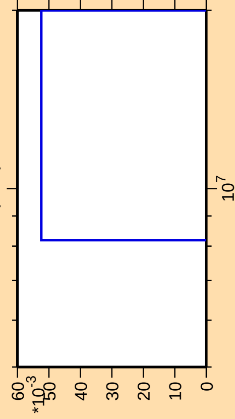
\Delta\sigma/\sigma vs. E for ^{49}\text{Sc}(n,nt)
