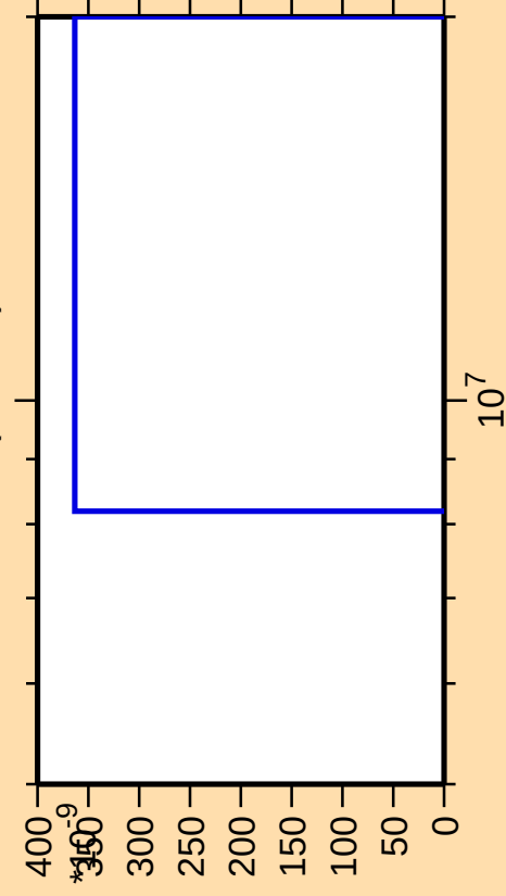
\Delta\sigma/\sigma vs. E for ^{49}\text{Sc}(n,\text{He}3)
