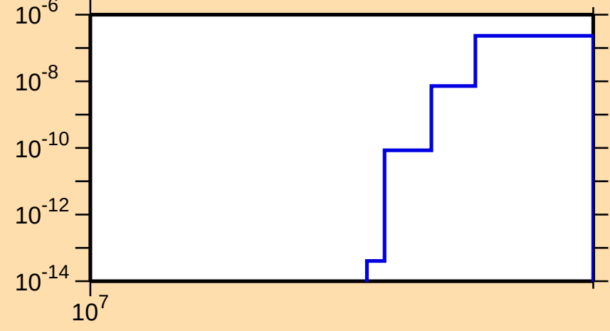
\sigma vs. E for ^{68}\text{Se}(n,\text{pt})
