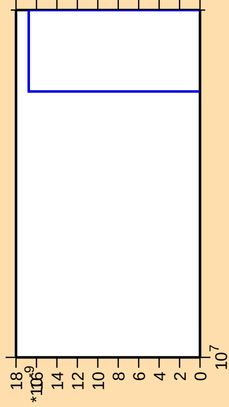
\Delta\sigma/\sigma vs. E for ^{68}\text{Se}(n,2n\alpha)
