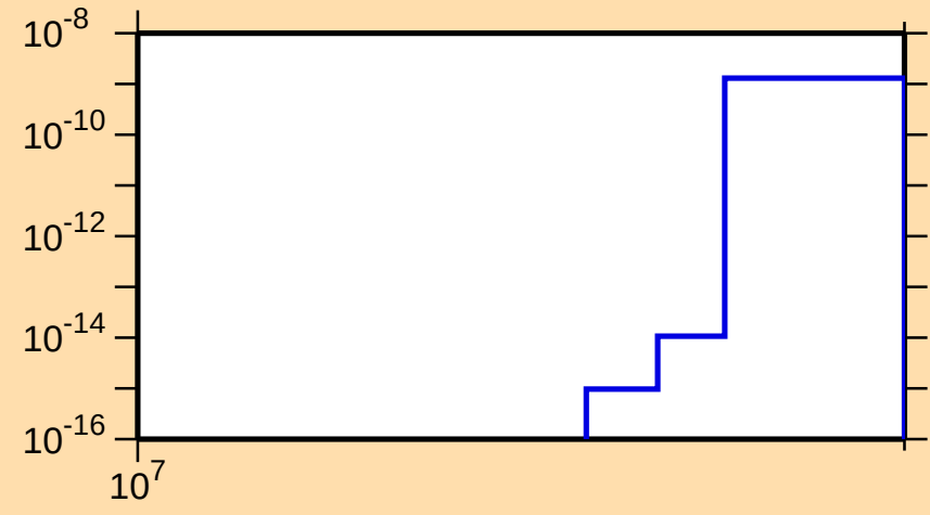
\sigma vs. E for ^{68}\text{Se}(n,\text{nd})
