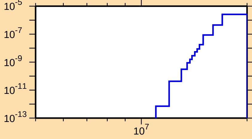
\sigma vs. E for ^{68}\text{Se}(\text{mt117})
