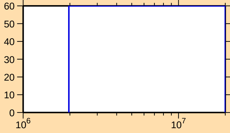
\Delta\sigma/\sigma vs. E for ^{68}\text{Se}(n,n\text{cont.})
