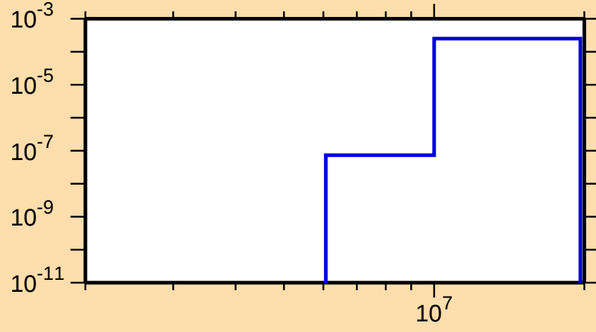
\sigma vs. E for ^{68}\text{Se}(n,n\alpha)
