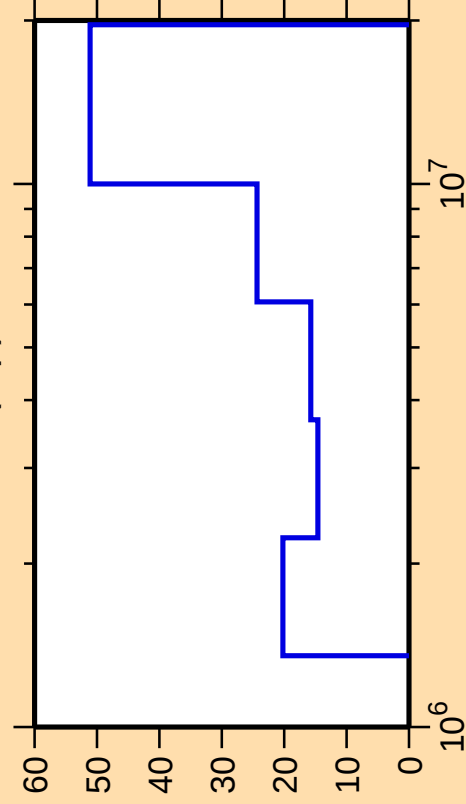
\Delta\sigma/\sigma vs. E for ^{68}\text{Se}(n,p)
