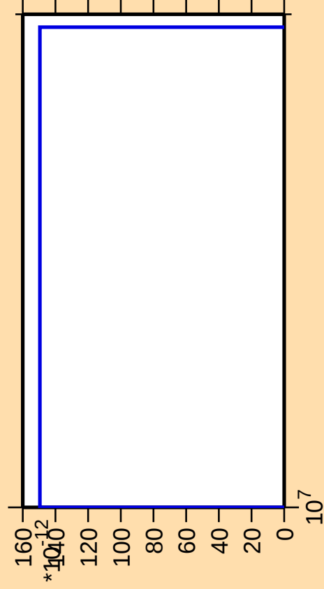
\Delta\sigma/\sigma vs. E for ^{68}\text{Se}(n,2n\alpha)
