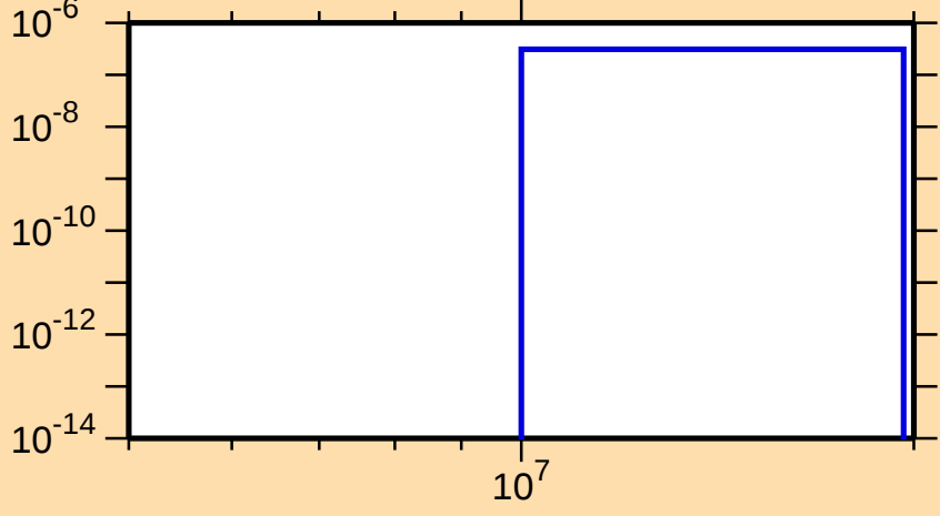
\sigma vs. E for ^{68}\text{Se}(n,t)
