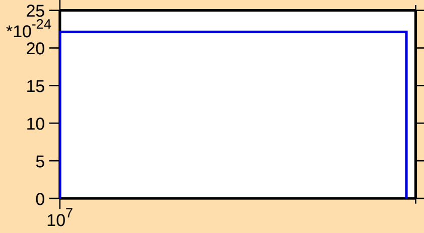
\sigma vs. E for ^{68}\text{Se}(n,2n\alpha)
