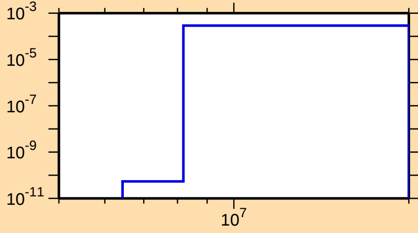
\sigma vs. E for ^{68}\text{Se}(n,\text{pd})
