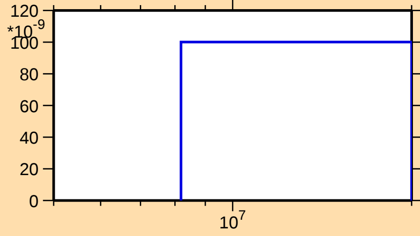
\sigma vs. E for ^{68}\text{Se}(\text{mt } 45)
