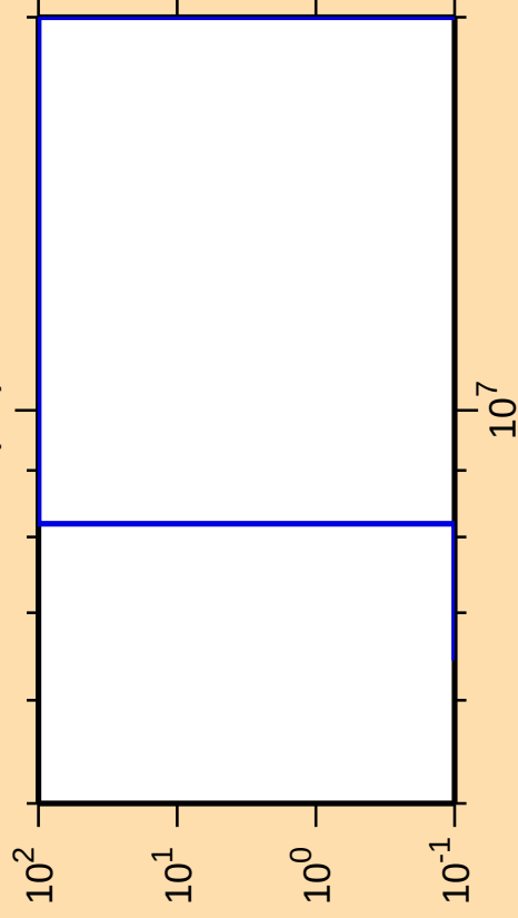
\Delta\sigma/\sigma vs. E for ^{69}\text{Se}(n,t)
