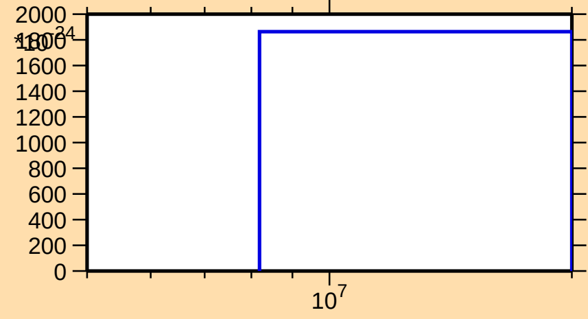
\sigma vs. E for ^{69}\text{Se}(n,nt)
