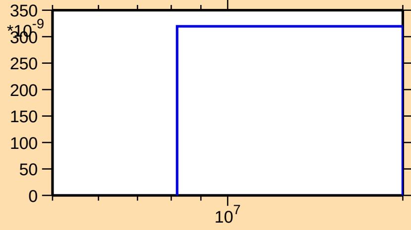
\sigma vs. E for ^{69}\text{Se}(\text{mt } 45)
