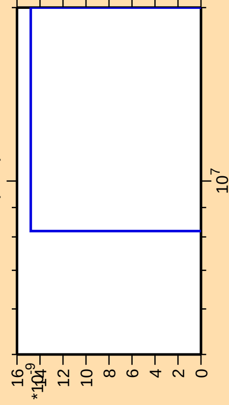
\Delta\sigma/\sigma vs. E for ^{69}\text{Se}(n,nt)
