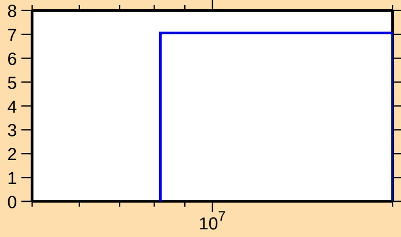
\Delta\sigma/\sigma vs. E for ^{69}\text{Se}(n,\text{tot.})
