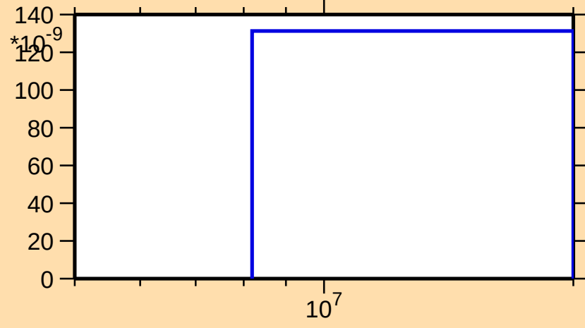
\sigma vs. E for ^{69}\text{Se}(\text{mt117})
