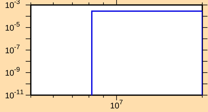
\sigma vs. E for ^{69}\text{Se}(n,t)
