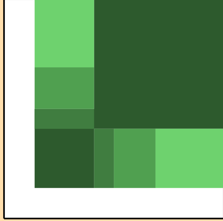
\sigma vs. E for ^{70}\text{Se}(n,np)
