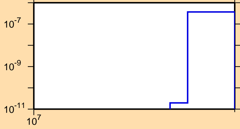
\sigma vs. E for ^{70}\text{Se}(n,\text{pt})
