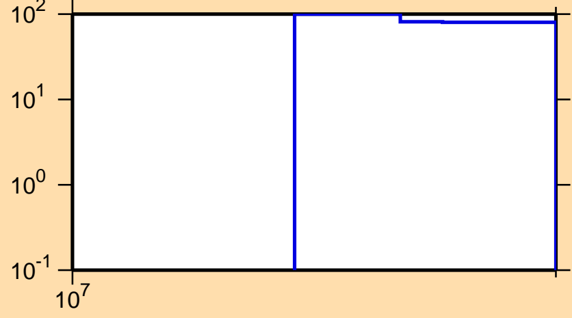
\Delta\sigma/\sigma vs. E for ^{70}\text{Se}(n,2n)
