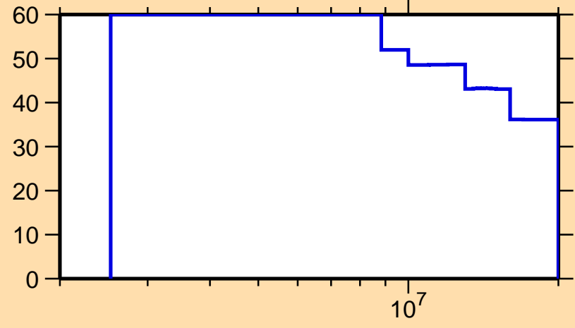
\Delta\sigma/\sigma vs. E for ^{70}\text{Se}(n,n\text{cont.})
