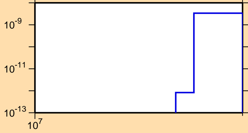
\sigma vs. E for ^{70}\text{Se}(n,\text{nd})
