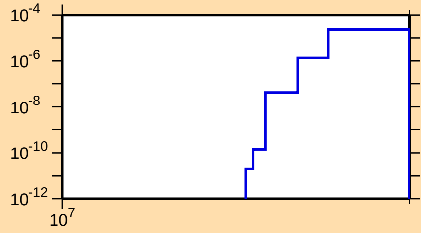
\sigma vs. E for ^{71}\text{Se}(n,\text{nd})
