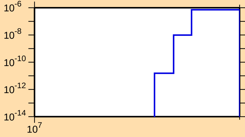
\sigma vs. E for ^{71}\text{Se}(n,2n\alpha)
