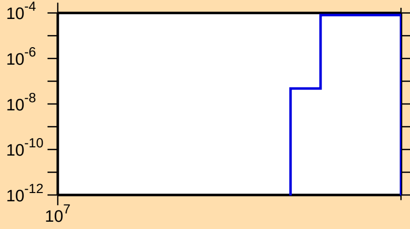
\sigma vs. E for ^{71}\text{Se}(n,2np)
