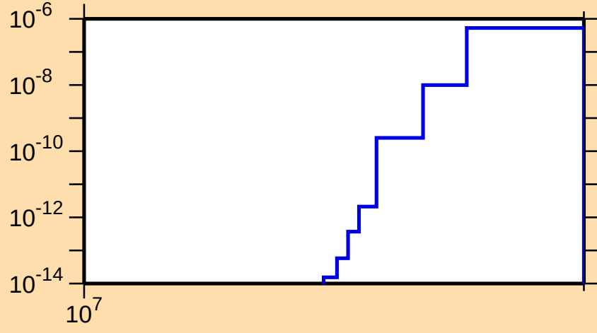
\sigma vs. E for ^{71}\text{Se}(\text{mt } 34)
