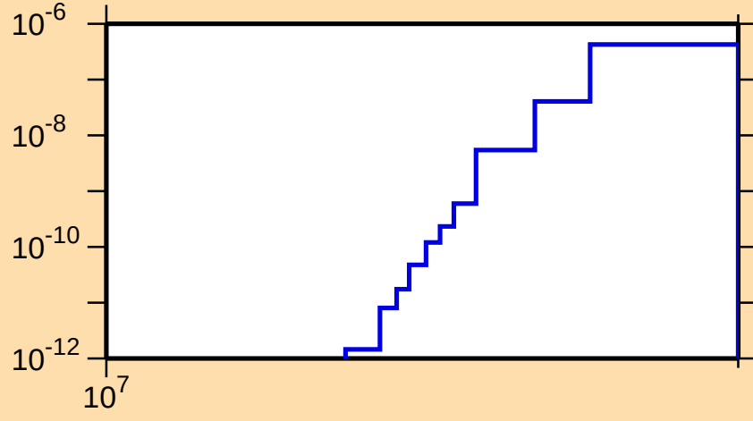
\sigma vs. E for ^{71}\text{Se}(\text{mt117})
