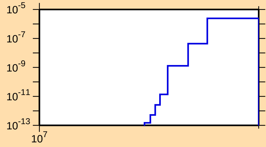
\sigma vs. E for ^{71}\text{Se}(\text{mt 45})
