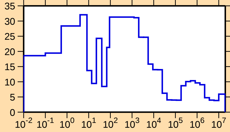
\Delta\sigma/\sigma vs. E for ^{71}\text{Se}(n,\text{tot.})
