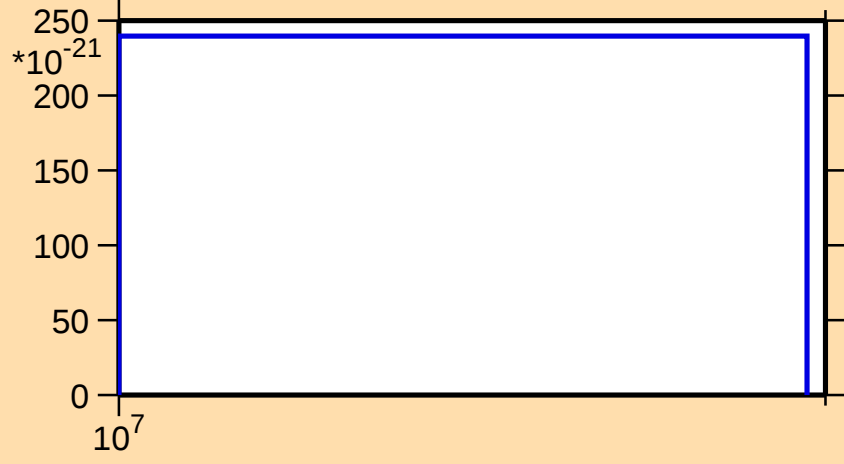
\sigma vs. E for ^{71}\text{Se}(n,\text{nt})
