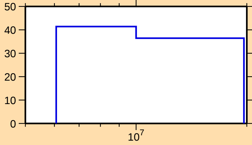
\Delta\sigma/\sigma vs. E for ^{71}\text{Se}(n,\text{inel.})
