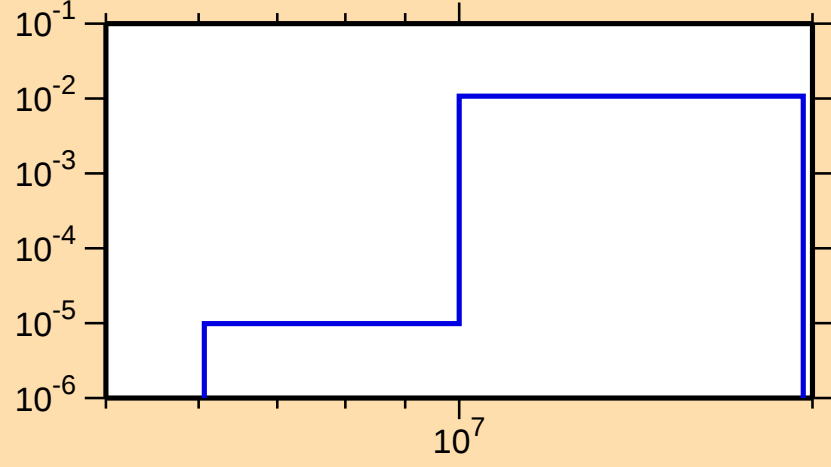
\sigma vs. E for ^{71}\text{Se}(n,2n)
