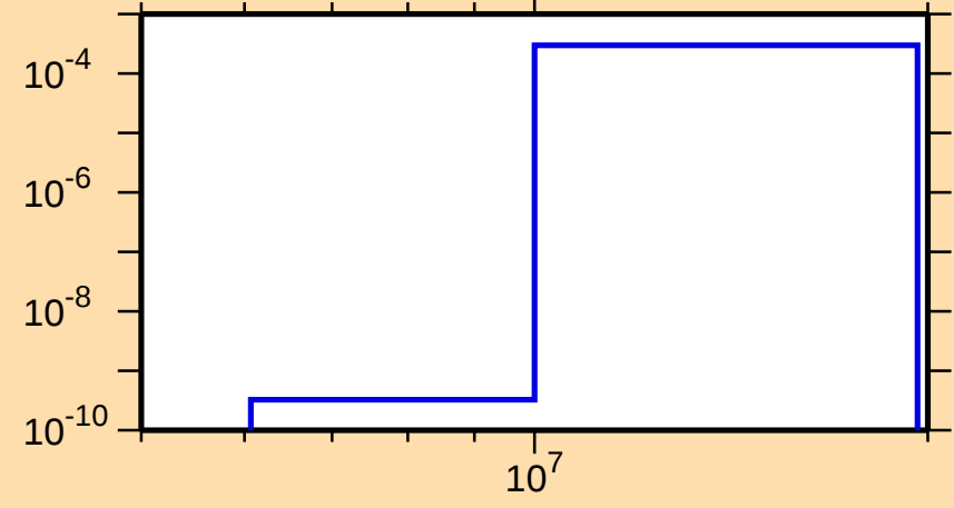
\sigma vs. E for ^{71}\text{Se}(n,t)
