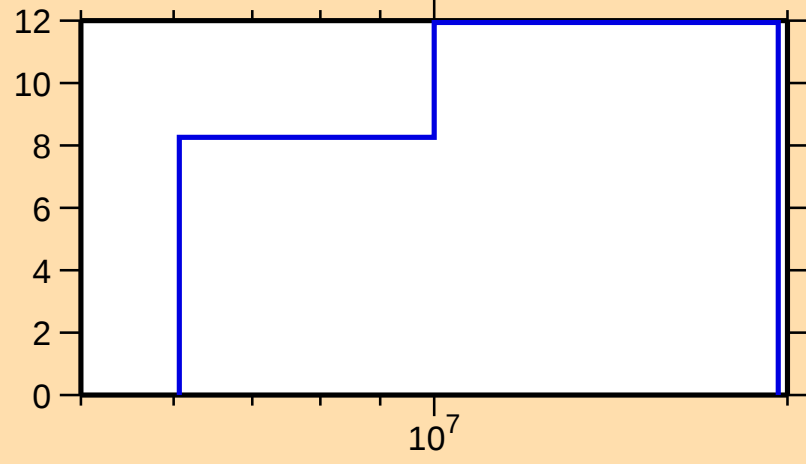
\Delta\sigma/\sigma vs. E for ^{71}\text{Se}(n,\text{el.})
