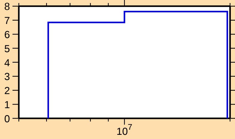
\Delta\sigma/\sigma vs. E for ^{71}\text{Se}(n,\text{nonel.})
