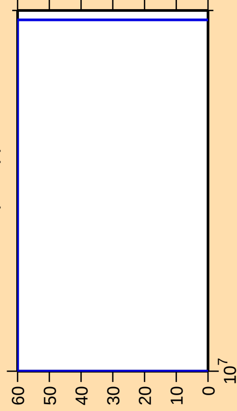
\Delta\sigma/\sigma vs. E for ^{71}\text{Se}(n,2np)
