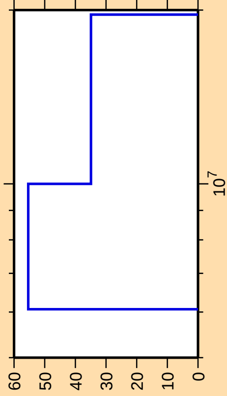
\Delta\sigma/\sigma vs. E for ^{71}\text{Se}(n,np)
