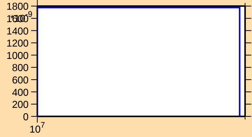
\sigma vs. E for ^{71}\text{Se}(n,\text{pt})
