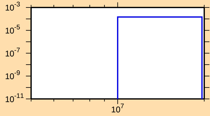
\sigma vs. E for ^{71}\text{Se}(n,\text{pd})
