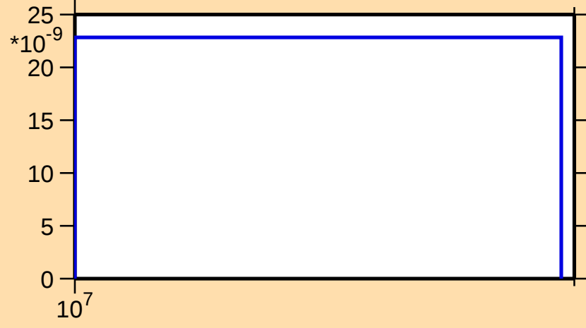
\sigma vs. E for ^{71}\text{Se}(\text{mt 45})
