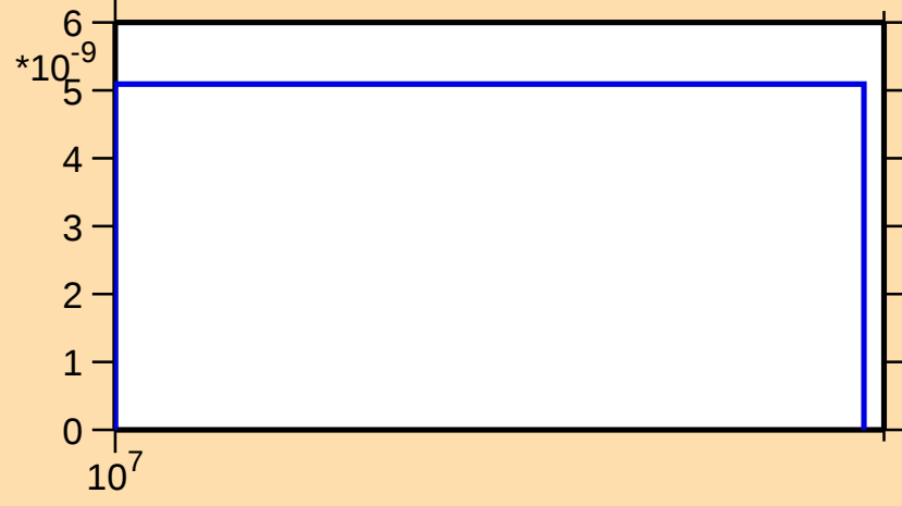
\sigma vs. E for ^{71}\text{Se}(\text{mt } 34)
