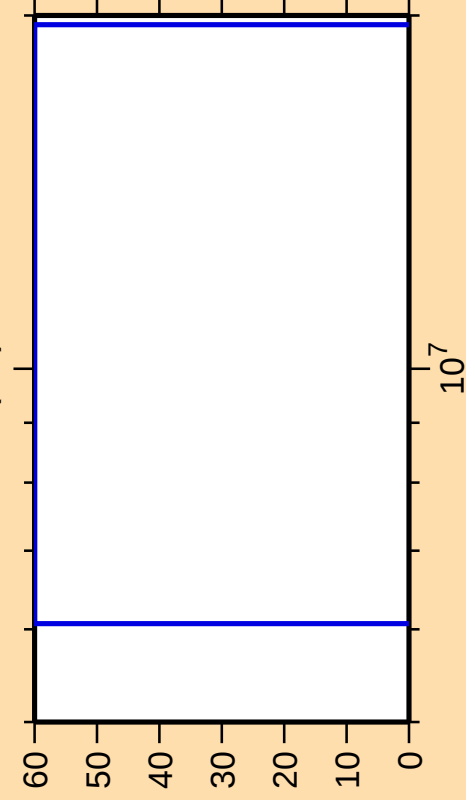
\Delta\sigma/\sigma vs. E for ^{71}\text{Se}(n,t)
