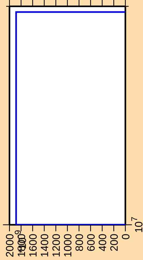
\Delta\sigma/\sigma vs. E for ^{71}\text{Se}(n,\text{nt})
