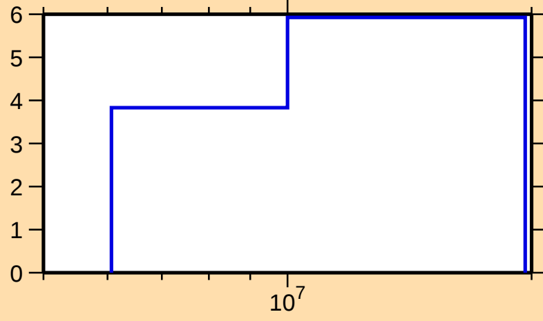
\Delta\sigma/\sigma vs. E for ^{71}\text{Se}(n,\text{tot.})
