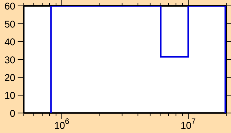
\Delta\sigma/\sigma vs. E for ^{71}\text{Se}(n,n\text{cont.})
