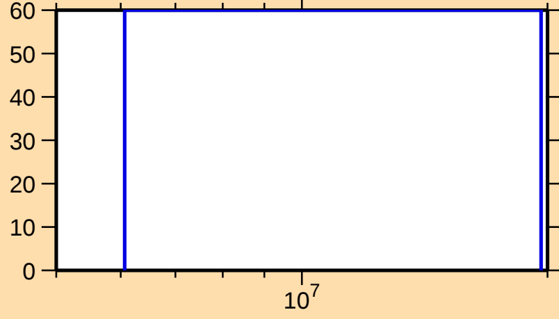
\Delta\sigma/\sigma vs. E for ^{71}\text{Se}(n,2n)
