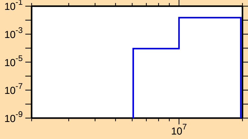
\sigma vs. E for ^{71}\text{Se}(n,n\alpha)
