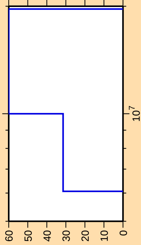
\Delta\sigma/\sigma vs. E for ^{71}\text{Se}(n,n\text{cont.})
