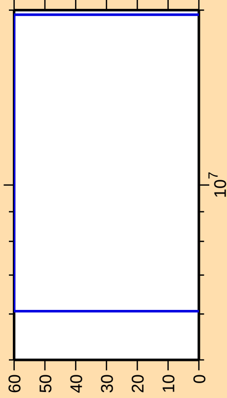
\Delta\sigma/\sigma vs. E for ^{71}\text{Se}(n,p)
