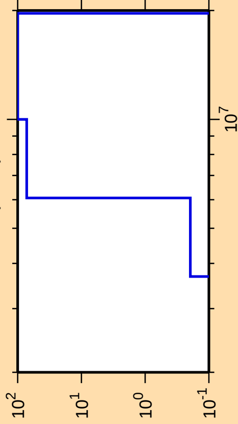
\Delta\sigma/\sigma vs. E for ^{71}\text{Se}(n,n\alpha)
