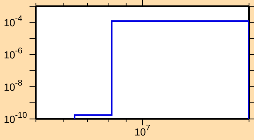
\sigma vs. E for ^{71}\text{Se}(n,\text{He3})
