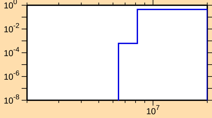
\sigma vs. E for ^{71}\text{Se}(n,np)
