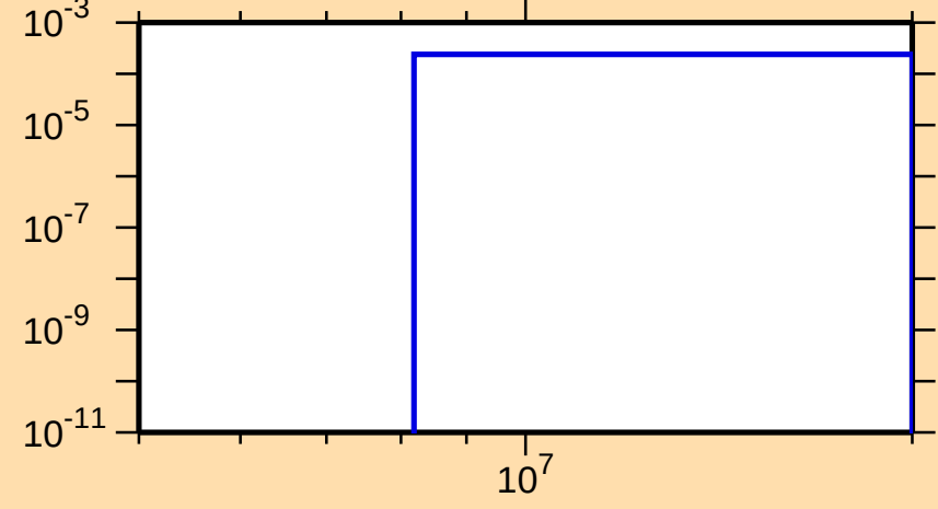
\sigma vs. E for ^{71}\text{Se}(n,t)
