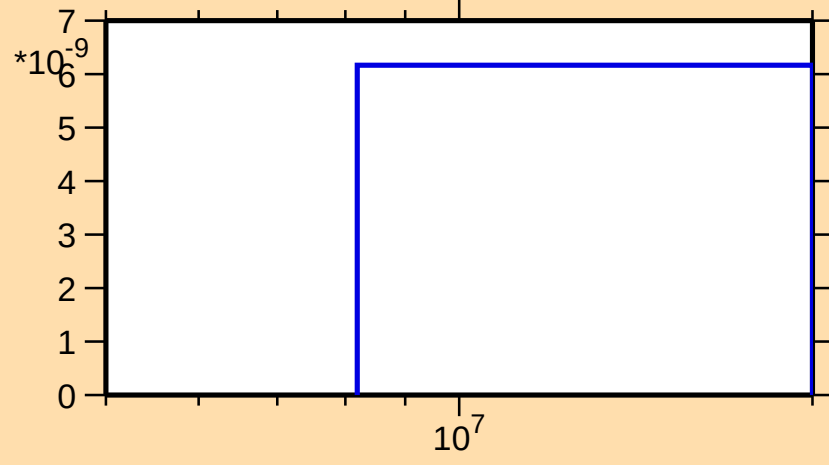
\sigma vs. E for ^{71}\text{Se}(n,2n\alpha)
