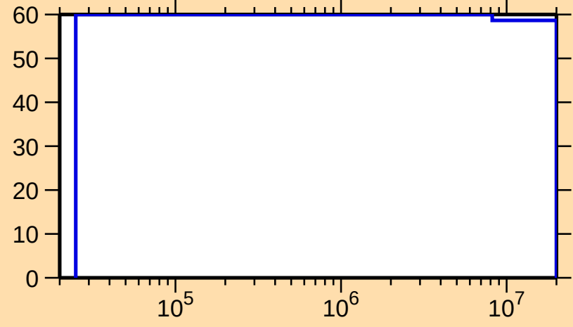
\Delta\sigma/\sigma vs. E for ^{71}\text{Se}(n,n_1)
