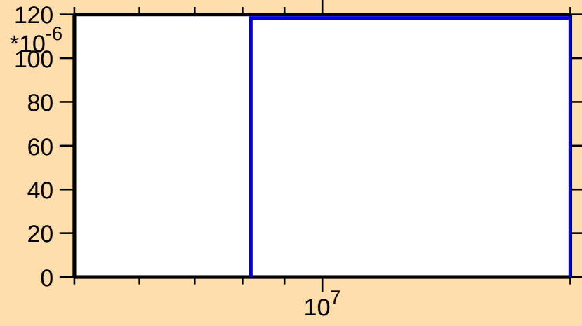
\sigma vs. E for ^{71}\text{Se}(n,\text{pd})
