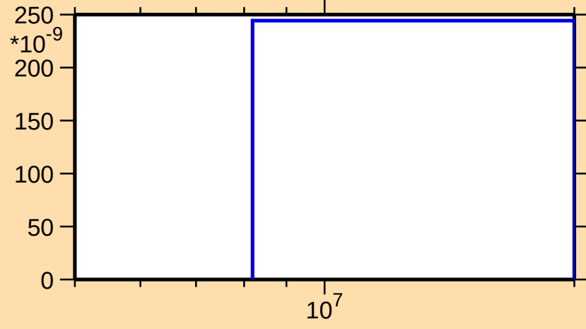
\sigma vs. E for ^{71}\text{Se}(n,\text{nd})
