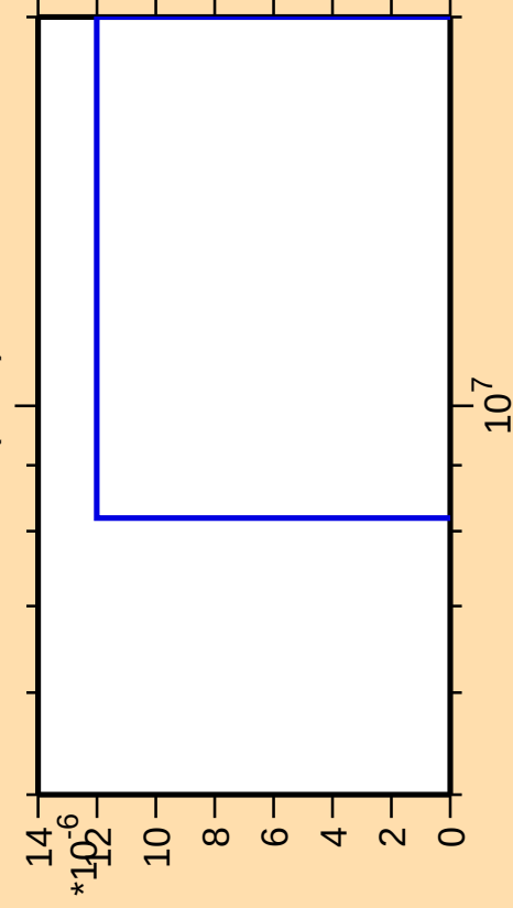
\Delta\sigma/\sigma vs. E for ^{71}\text{Se}(n,\text{nt})
