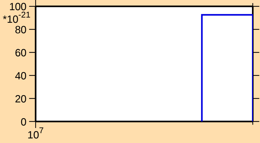
\sigma vs. E for ^{73}\text{Se}(n,\text{nt})
