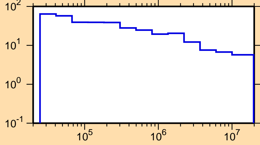
\Delta\sigma/\sigma vs. E for ^{73}\text{Se}(n,\text{nonel.})
