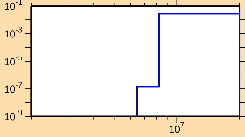
\sigma vs. E for ^{73}\text{Se}(n,n\alpha)
