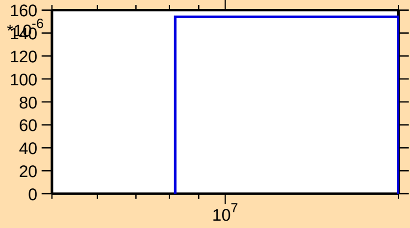
\sigma vs. E for ^{73}\text{Se}(n,t)
