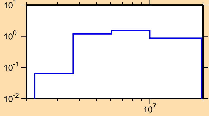
\sigma vs. E for ^{74}\text{Se}(n,n\text{cont.})
