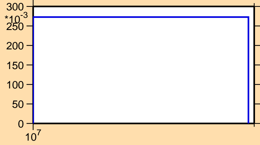
\sigma vs. E for ^{74}\text{Se}(n,2n)
