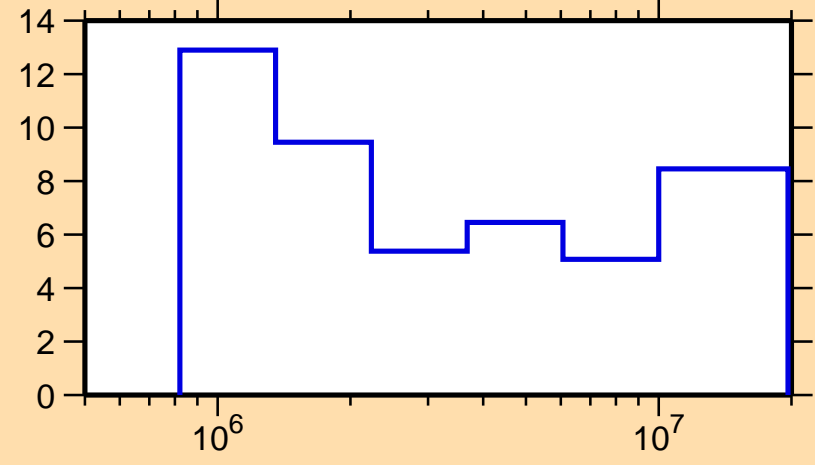
\Delta\sigma/\sigma vs. E for ^{74}\text{Se}(n,el.)
