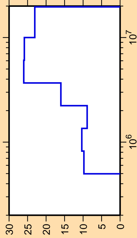
\Delta\sigma/\sigma vs. E for ^{74}\text{Se}(n,n_1)
