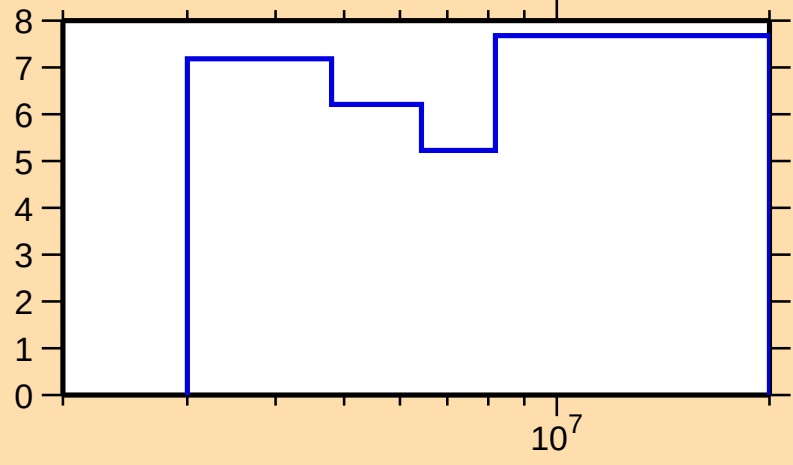
\Delta\sigma/\sigma vs. E for ^{74}\text{Se}(n,\text{el.})
