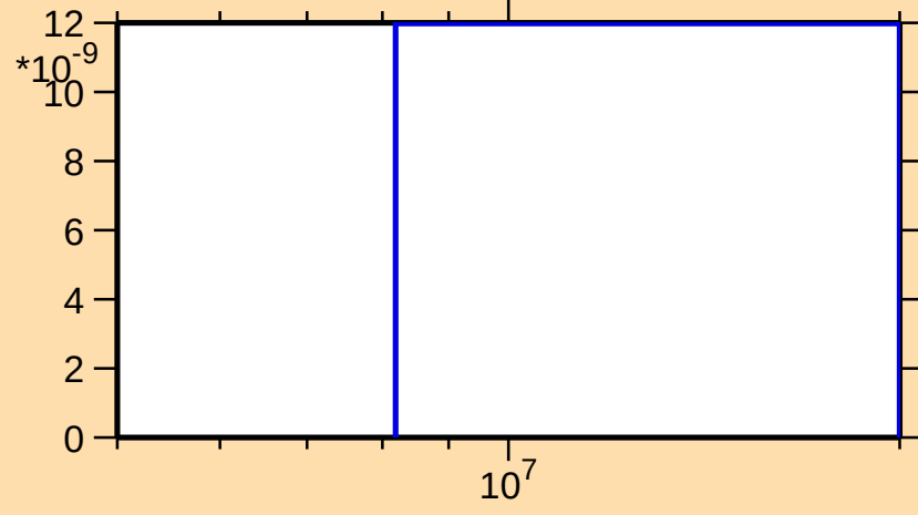
\sigma vs. E for ^{74}\text{Se}(n,\text{pd})
