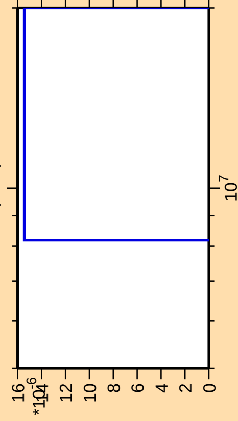
\Delta\sigma/\sigma vs. E for ^{74}\text{Se}(n,nt)
