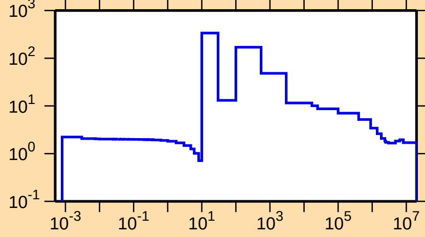
\sigma vs. E for ^{74}\text{Se}(n,\text{el.})
