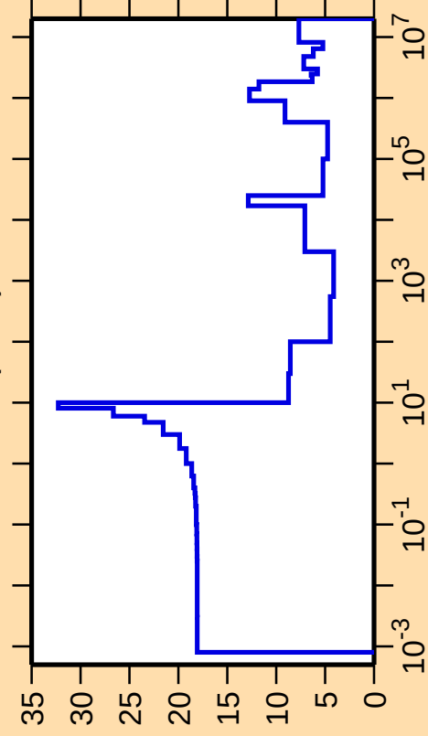
\Delta\sigma/\sigma vs. E for ^{74}\text{Se}(n,\text{el.})
