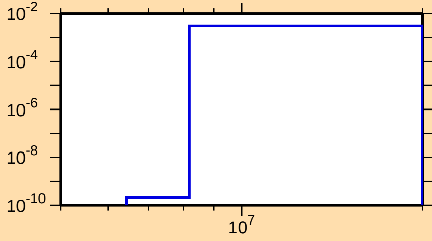
\sigma vs. E for ^{74}\text{Se}(n,d)
