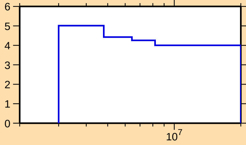
\Delta\sigma/\sigma vs. E for ^{74}\text{Se}(n,n\text{nonel.})
