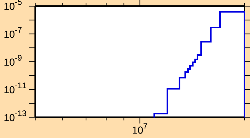
\sigma vs. E for ^{75}\text{Se}(n,\text{He3})
