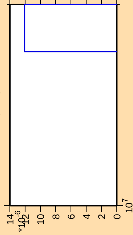
\Delta\sigma/\sigma vs. E for ^{75}\text{Se}(n,\text{nt})
