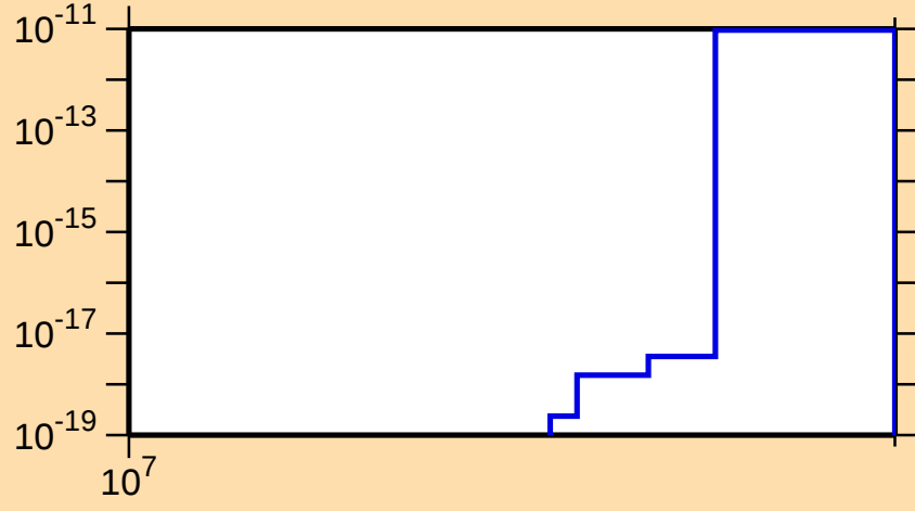
\sigma vs. E for ^{75}\text{Se}(\text{mt } 34)
