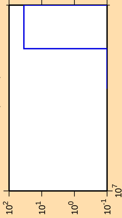
\Delta\sigma/\sigma vs. E for ^{75}\text{Se}(\text{mt } 34)
