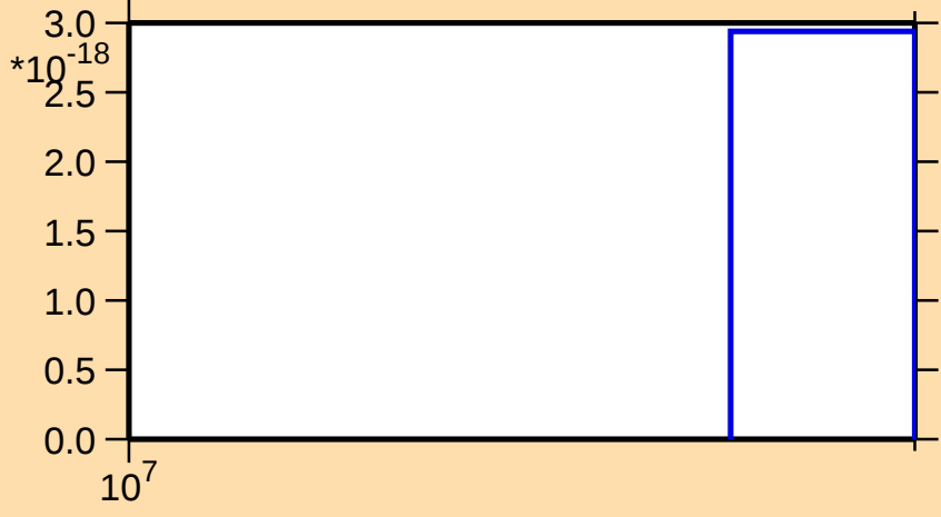
\sigma vs. E for ^{75}\text{Se}(n,\text{nt})
