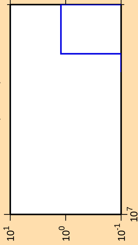
\Delta\sigma/\sigma vs. E for ^{75}\text{Se}(\text{mt117})
