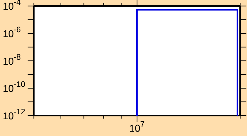
\sigma vs. E for ^{75}\text{Se}(n,t)
