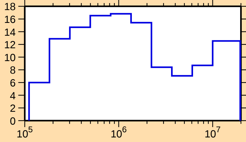
\Delta\sigma/\sigma vs. E for ^{75}\text{Se}(\text{n,el.})
