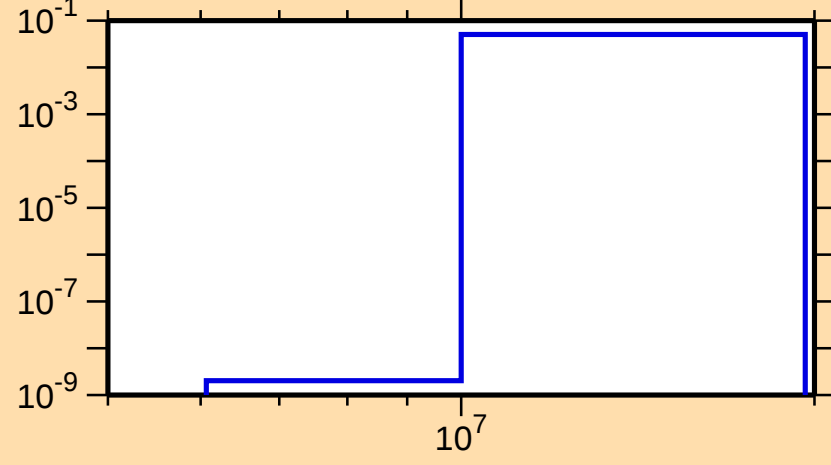
\sigma vs. E for ^{75}\text{Se}(n,np)
