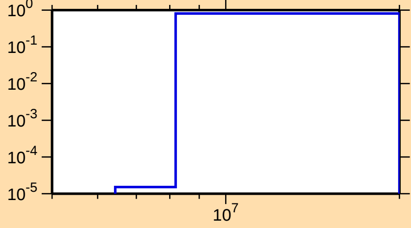
\sigma vs. E for ^{75}\text{Se}(n,2n)
