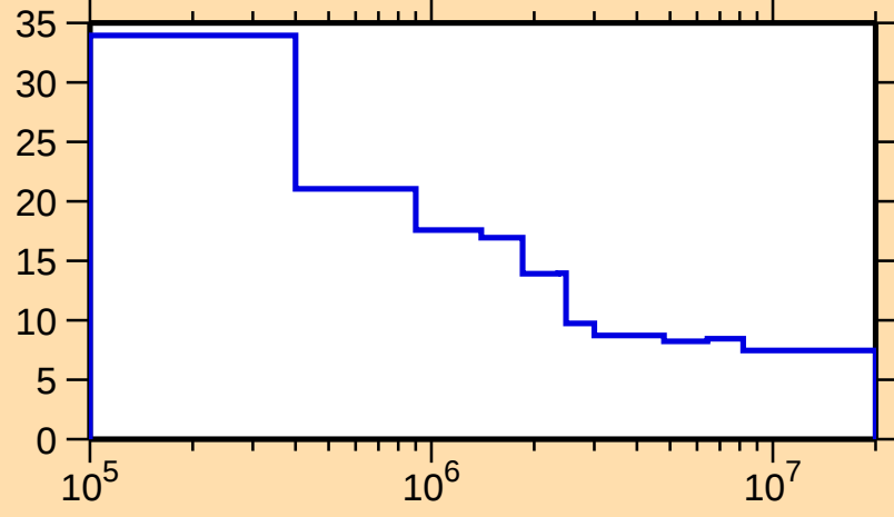
\Delta\sigma/\sigma vs. E for ^{75}\text{Se}(\text{n,nonel.})
