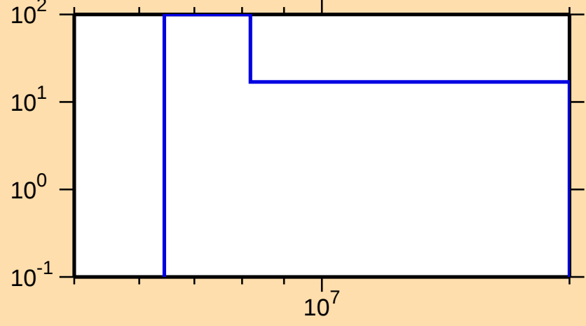
\Delta\sigma/\sigma vs. E for ^{75}\text{Se}(n,2n)
