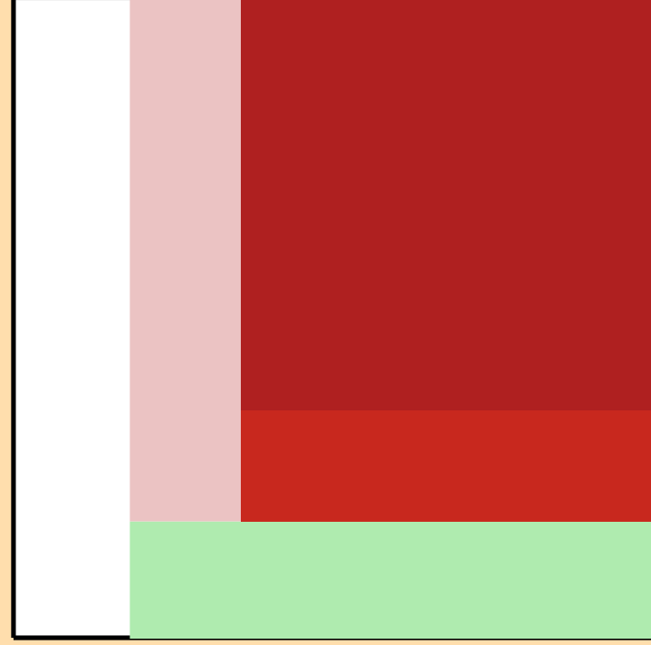
\Delta\sigma/\sigma vs. E for ^{75}\text{Se}(n,2n)
