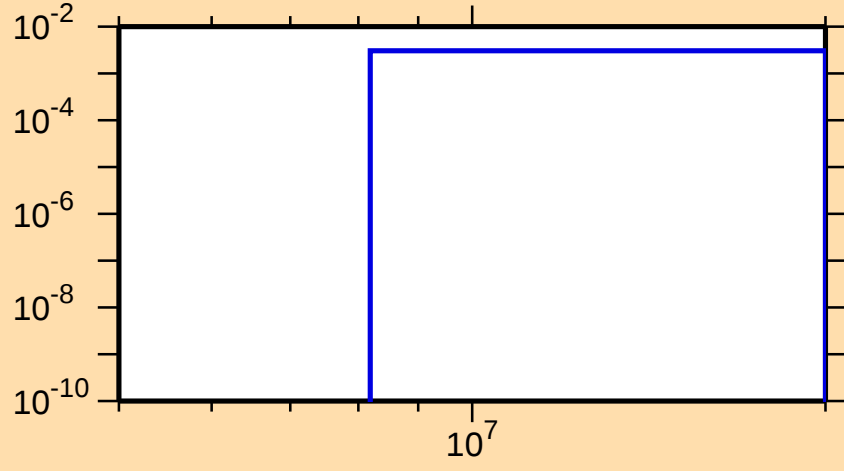
\sigma vs. E for ^{75}\text{Se}(n,d)
