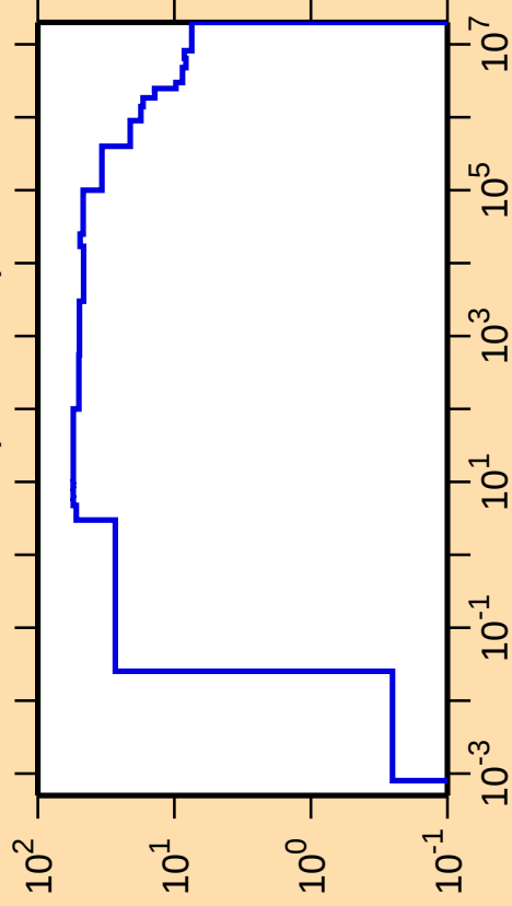
\Delta\sigma/\sigma vs. E for ^{75}\text{Se}(n,\text{nonel.})
