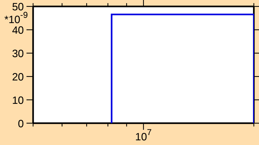
\sigma vs. E for ^{75}\text{Se}(n,\text{He3})
