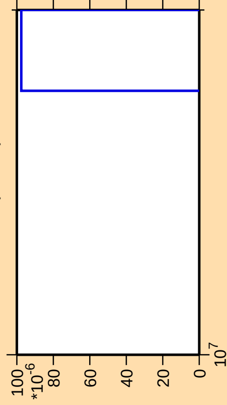
\Delta\sigma/\sigma vs. E for ^{76}\text{Se}(\text{mt 34})
