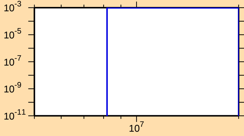
\sigma vs. E for ^{76}\text{Se}(n,n\alpha)
