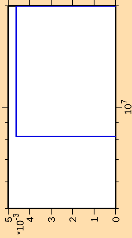
\Delta\sigma/\sigma vs. E for ^{76}\text{Se}(n,2n\alpha)
