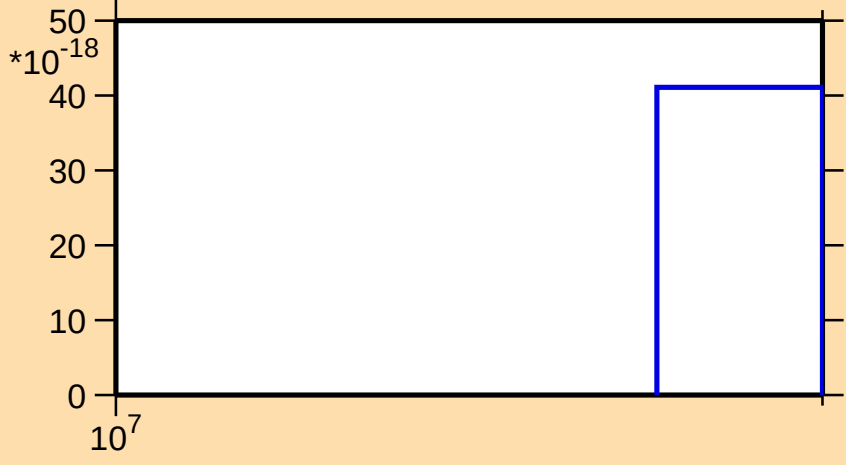
\sigma vs. E for ^{77}\text{Se}(n,\text{nt})
