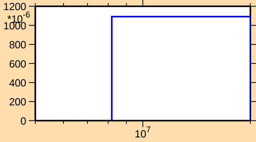
\sigma vs. E for ^{77}\text{Se}(n,n\alpha)
