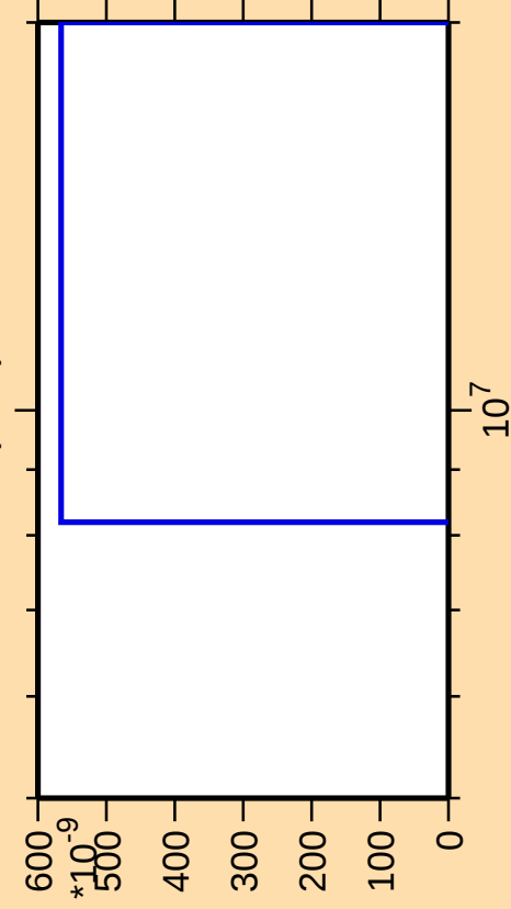
\Delta\sigma/\sigma vs. E for ^{77}\text{Se}(n,\text{nt})
