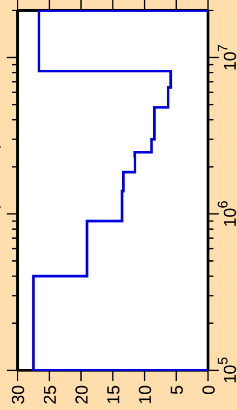
\Delta\sigma/\sigma vs. E for ^{77}\text{Se}(\text{n,inel.})
