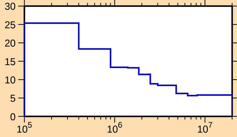
\Delta\sigma/\sigma vs. E for ^{77}\text{Se}(\text{n,nonel.})
