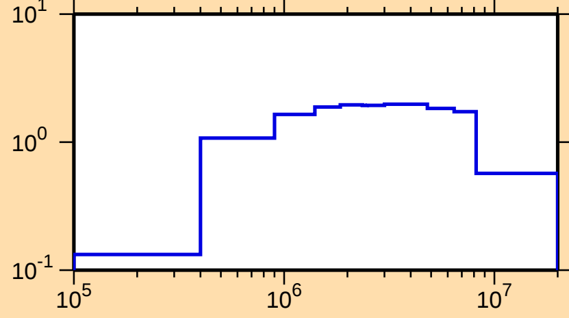
\sigma vs. E for ^{77}\text{Se}(n,\text{inel.})
