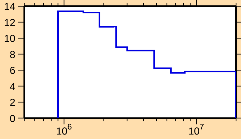
\Delta\sigma/\sigma vs. E for ^{77}\text{Se}(n,n\text{oncl.})
