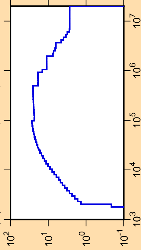
\Delta\mu/\mu vs. E for ^{78}\text{Se}(\text{mt251})
