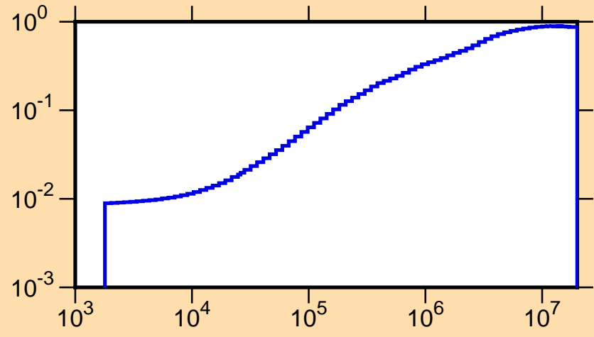
\mu vs. E for ^{78}\text{Se}(\text{mt251})
