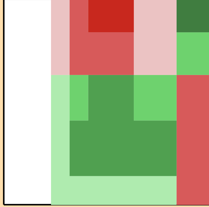
\Delta\sigma/\sigma vs. E for ^{79}\text{Se}(n,2n)
