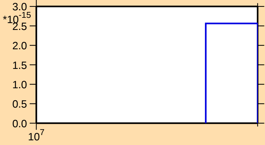
\sigma vs. E for ^{79}\text{Se}(n,\text{nt})
