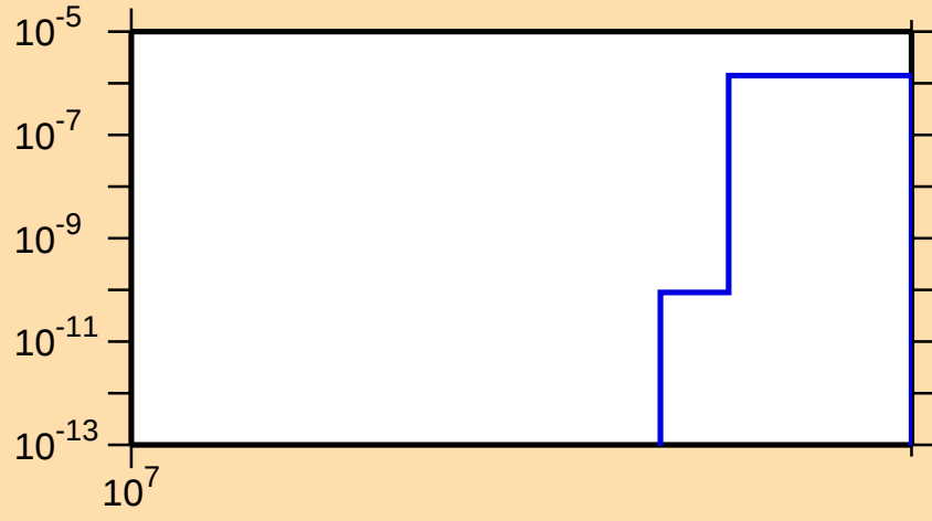
\sigma vs. E for ^{79}\text{Se}(n,\text{nd})
