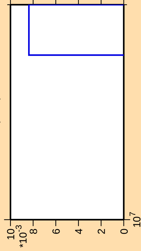
\Delta\sigma/\sigma vs. E for ^{79}\text{Se}(n,\text{nt})
