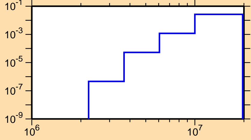
\sigma vs. E for ^{79}\text{Se}(n,p)
