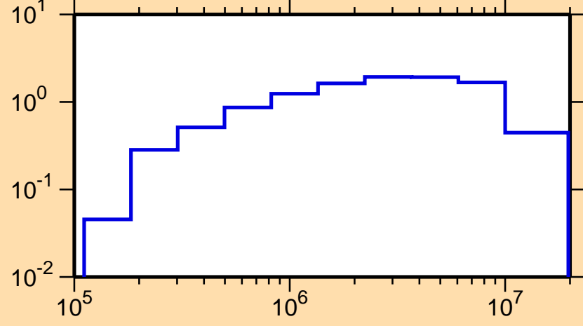
\sigma vs. E for ^{79}\text{Se}(n,\text{inel.})
