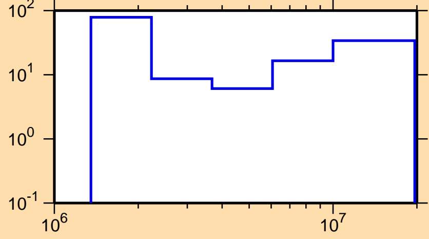
\Delta\sigma/\sigma vs. E for ^{79}\text{Se}(n,ncont.)
