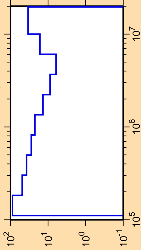
\Delta\sigma/\sigma vs. E for ^{79}\text{Se}(n,\text{inel.})
