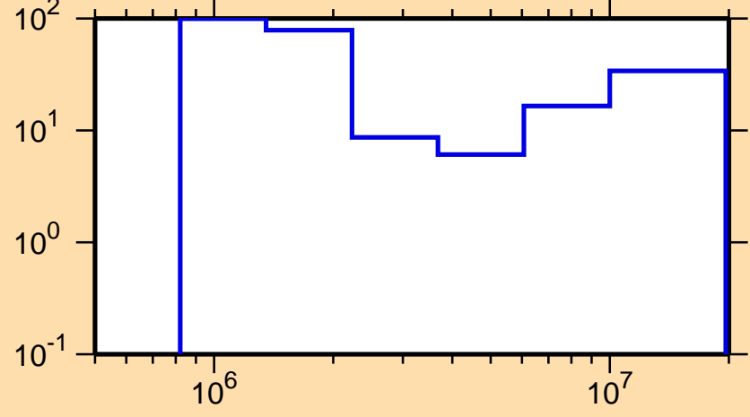
\Delta\sigma/\sigma vs. E for ^{79}\text{Se}(n,n\text{cont.})
