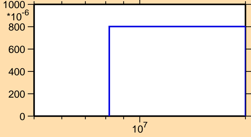
\sigma vs. E for ^{79}\text{Se}(n,d)
