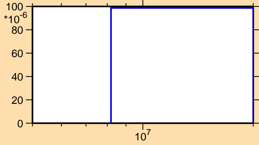
\sigma vs. E for ^{79}\text{Se}(n,t)
