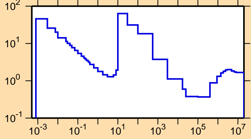
\sigma vs. E for ^{79}\text{Se}(n,\text{nonel.})
