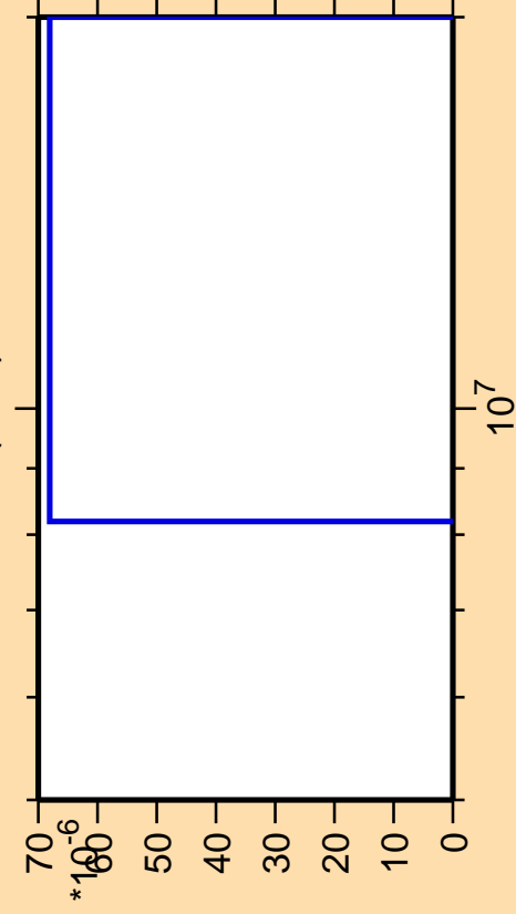
\Delta\sigma/\sigma vs. E for ^{79}\text{Se}(n,nt)
