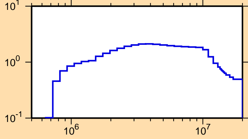
\sigma vs. E for ^{80}\text{Se}(n,\text{inel.})
