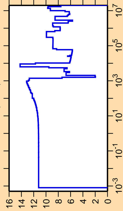
\Delta\sigma/\sigma vs. E for ^{80}\text{Se}(n,\text{el.})
