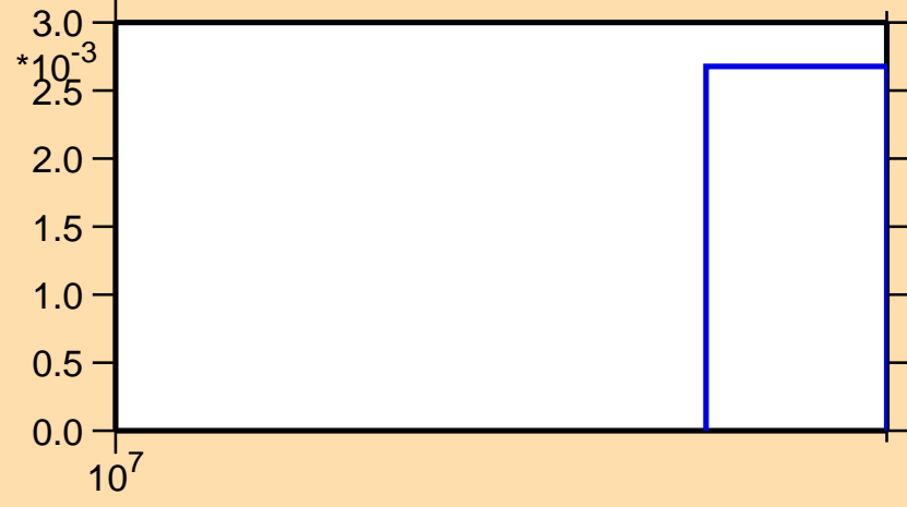
\sigma vs. E for ^{80}\text{Se}(n,3n)
