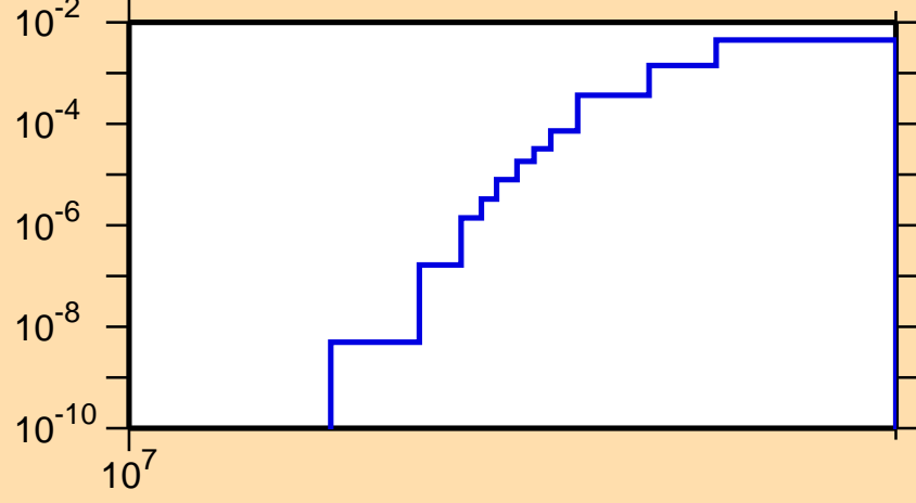
\sigma vs. E for ^{80}\text{Se}(n,np)
