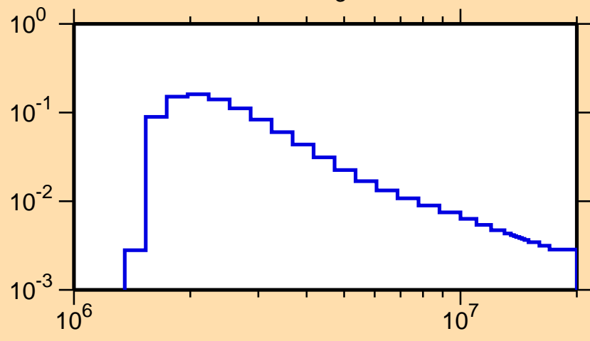
\sigma vs. E for ^{80}\text{Se}(n,n_3)
