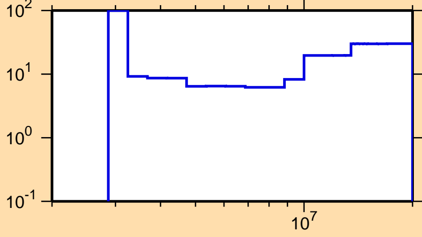
\Delta\sigma/\sigma vs. E for ^{80}\text{Se}(n,n\text{cont.})
