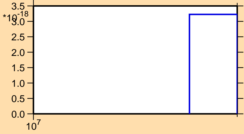
\sigma vs. E for ^{80}\text{Se}(n,nt)
