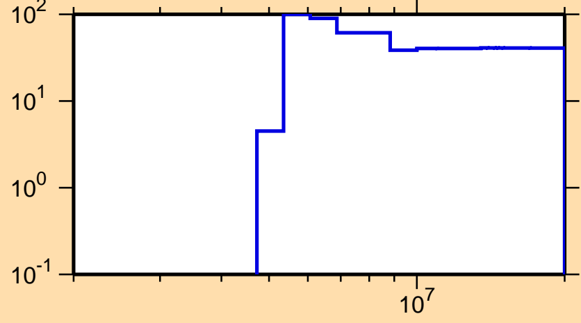
\Delta\sigma/\sigma vs. E for ^{80}\text{Se}(n,p)
