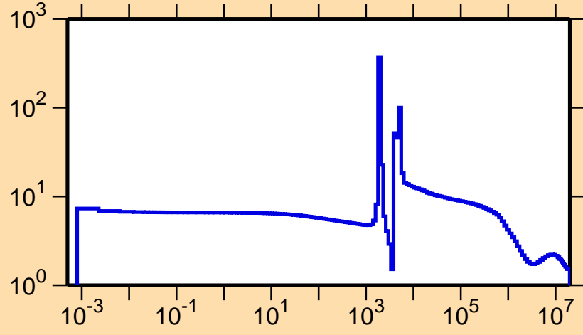
\sigma vs. E for ^{80}\text{Se}(n,\text{el.})
