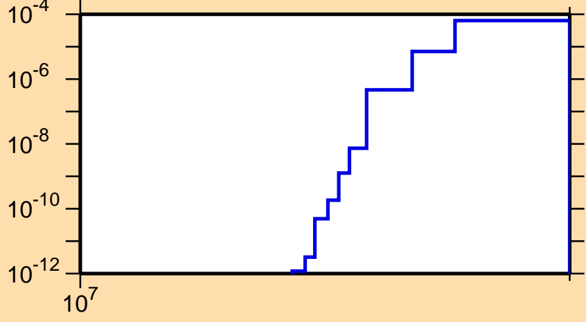
\sigma vs. E for ^{80}\text{Se}(n,t)
