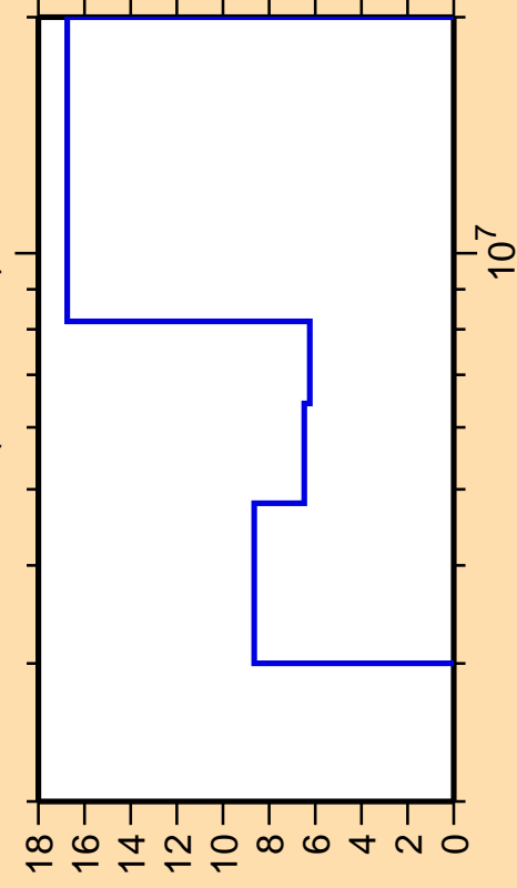
\Delta\sigma/\sigma vs. E for ^{80}\text{Se}(n,\text{ncont.})
