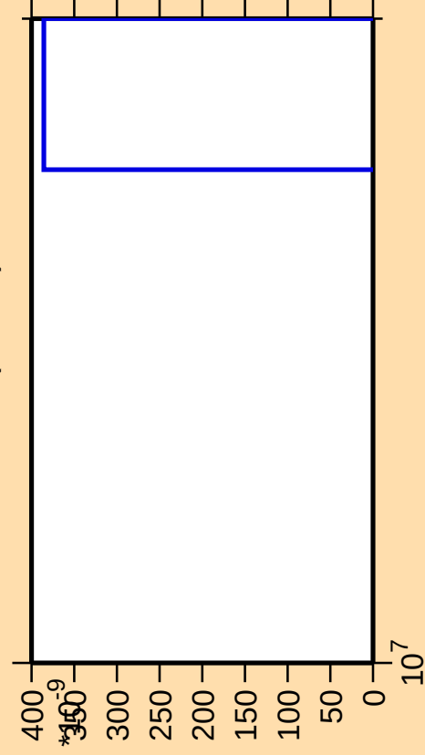
\Delta\sigma/\sigma vs. E for ^{81}\text{Se}(\text{mt } 34)
