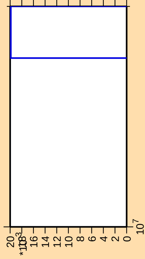
\Delta\sigma/\sigma vs. E for ^{81}\text{Se}(n,\text{He}3)
