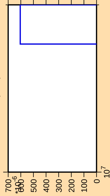
\Delta\sigma/\sigma vs. E for ^{81}\text{Se}(n,\text{nt})
