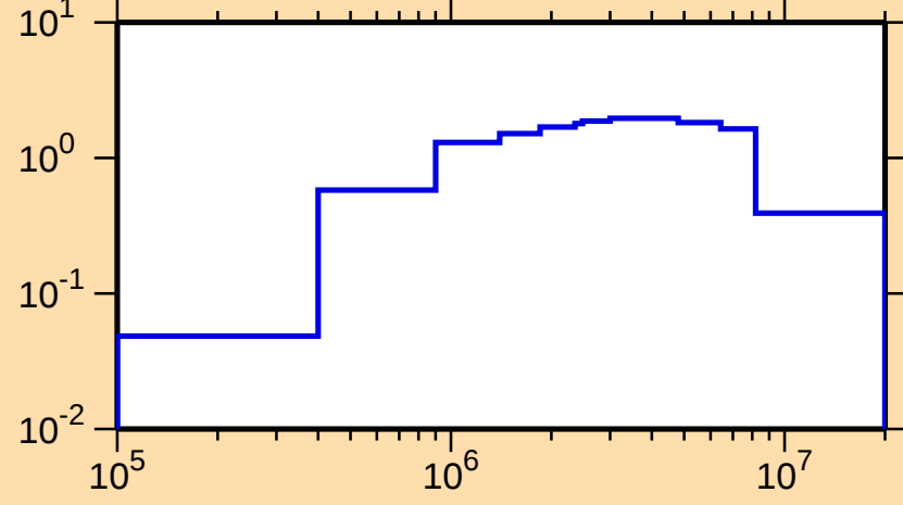
\sigma vs. E for ^{81}\text{Se}(n,\text{inel.})
