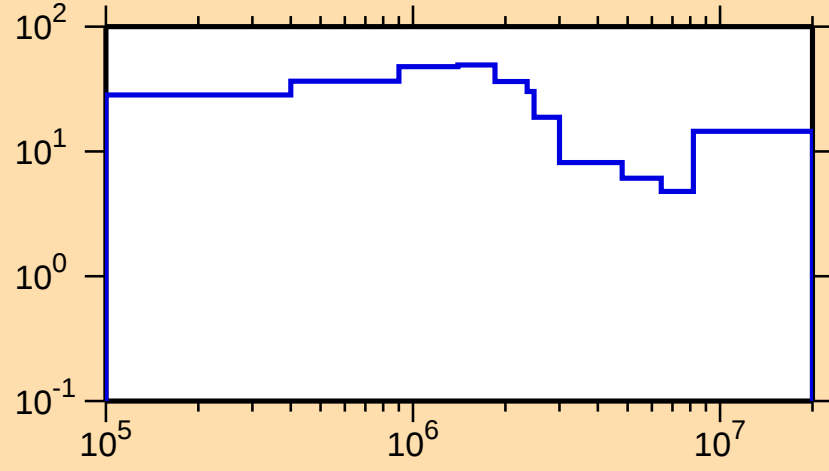
\Delta\sigma/\sigma vs. E for ^{81}\text{Se}(\text{n,el.})
