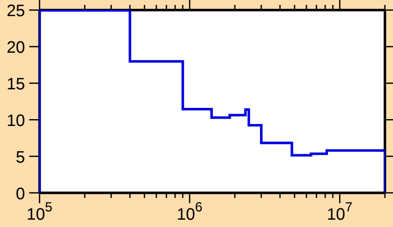
\Delta\sigma/\sigma vs. E for ^{81}\text{Se}(\text{n,nonel.})
