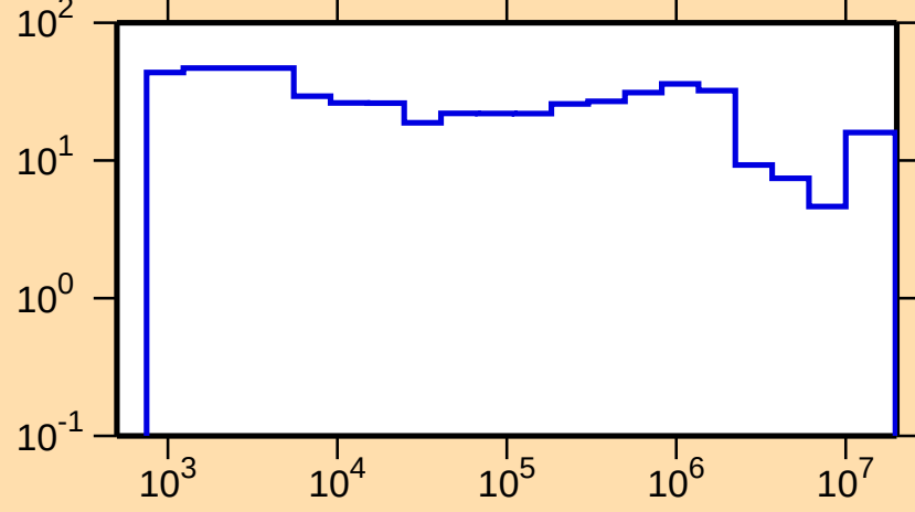
\Delta\sigma/\sigma vs. E for ^{81}\text{Se}(n,\text{el.})
