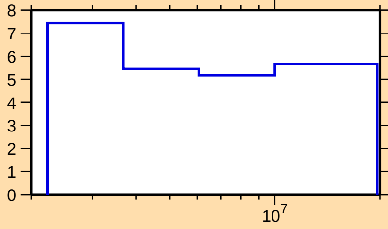
\Delta\sigma/\sigma vs. E for ^{81}\text{Se}(n,n\text{nonel.})
