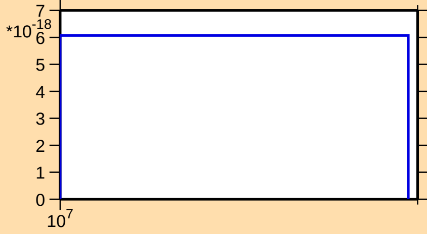
\sigma vs. E for ^{81}\text{Se}(n,\text{nt})
