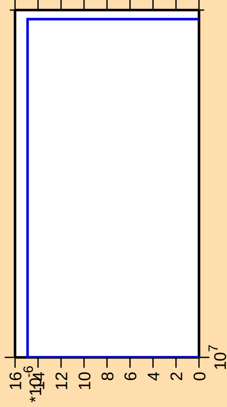
\Delta\sigma/\sigma vs. E for ^{81}\text{Se}(n,\text{nt})
